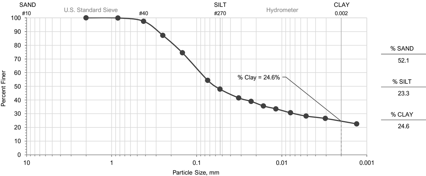
USDA Summation Curve Test Method: AASHTO T-88
