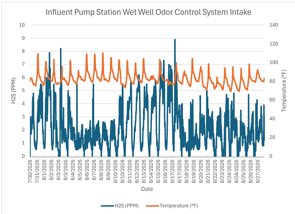
Monitor 1a Within WRF: Influent Pump Station Wet Well Odor Control System Intake H2S PPM August 2026.
