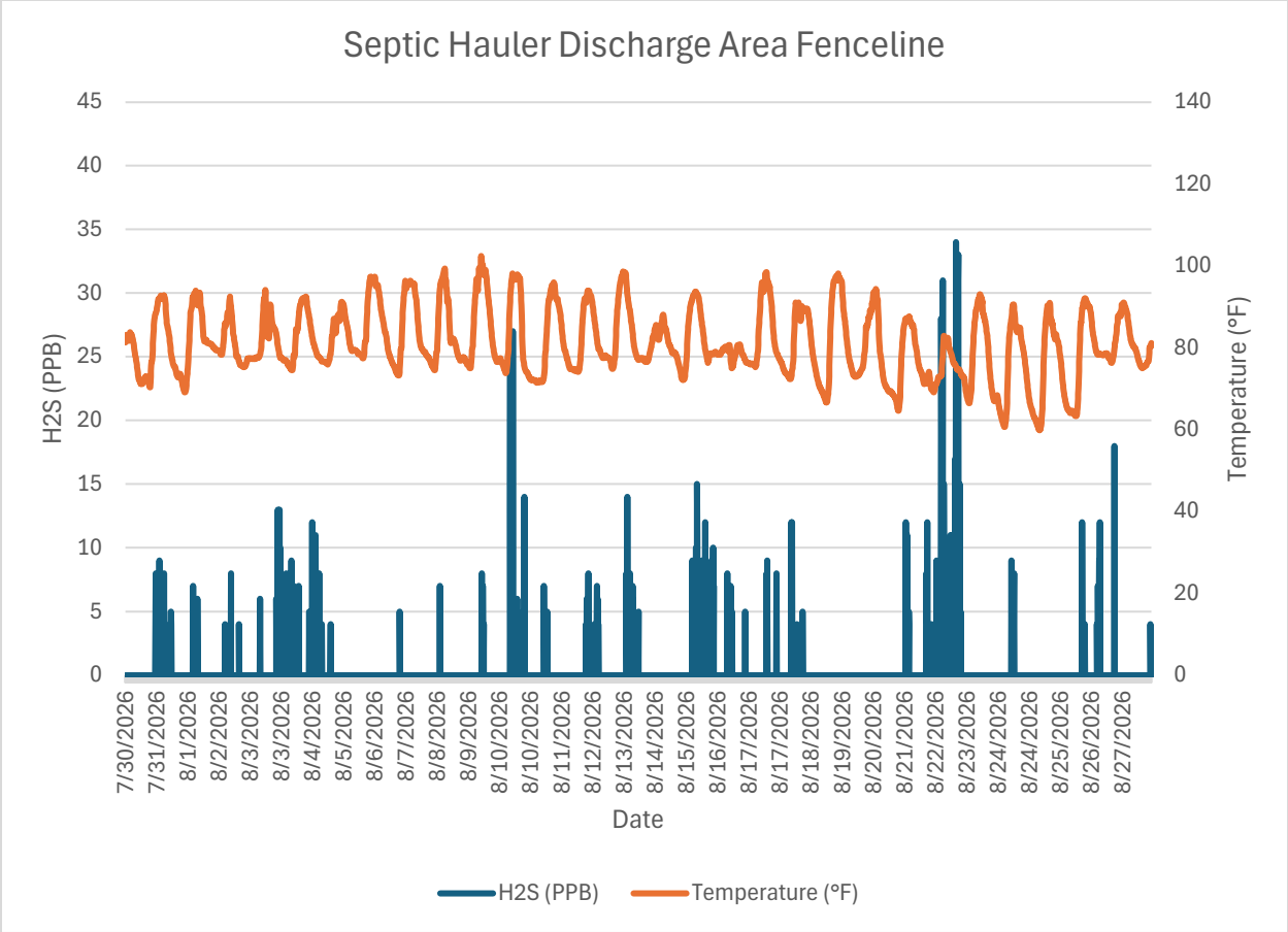
Monitor 1 Fenceline: Septic Hauler Discharge Area Fenceline H2S PPB August, 2026
