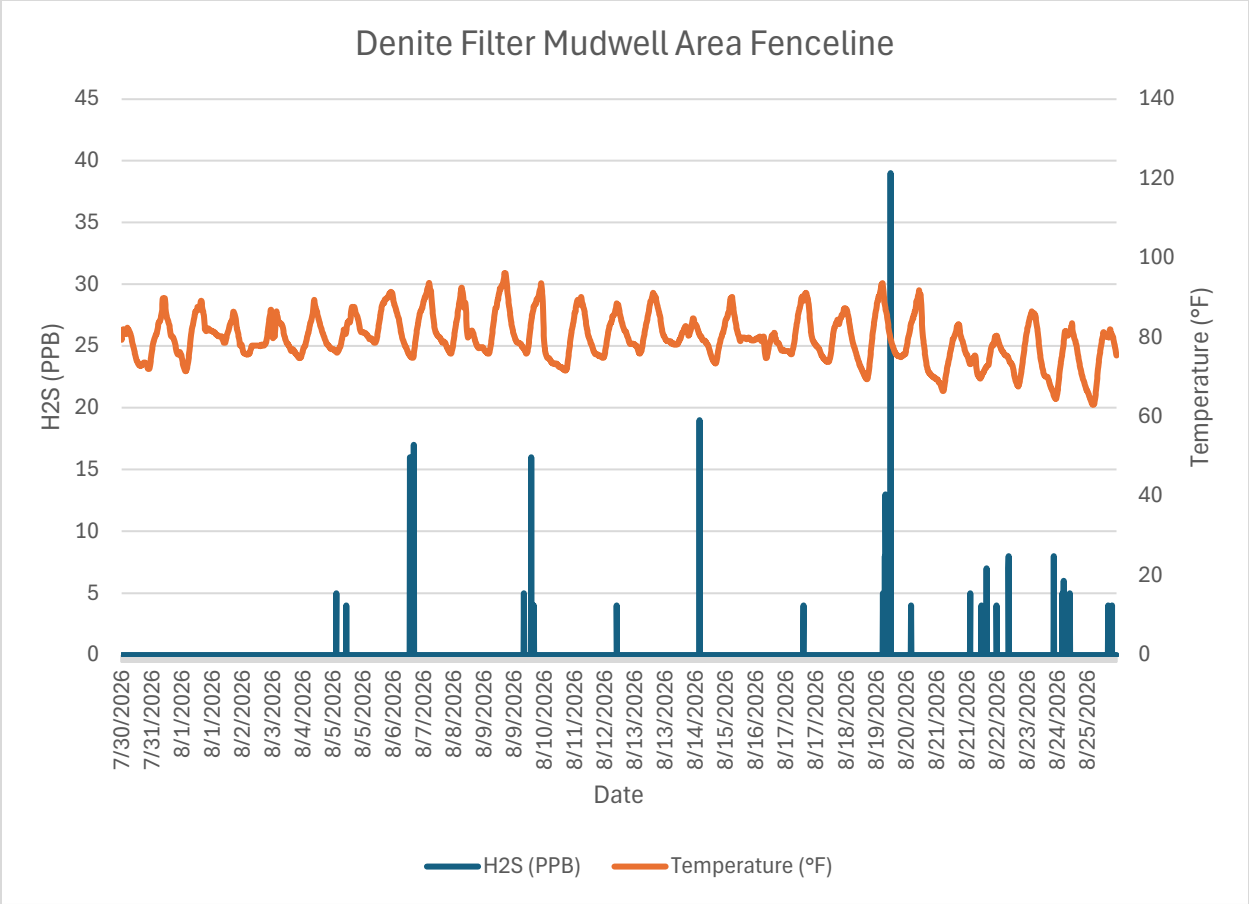
Monitor 3 Fenceline: Denite Filter Mudwell Area Fenceline H2S PPB August, 2026
