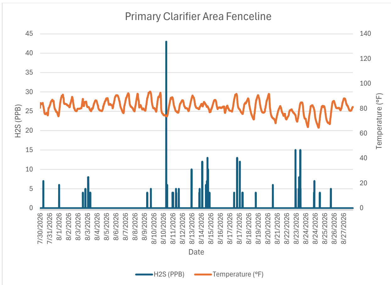
Monitor 2 Fenceline: Primary Clarifier Area Fenceline H2S PPB August, 2026
