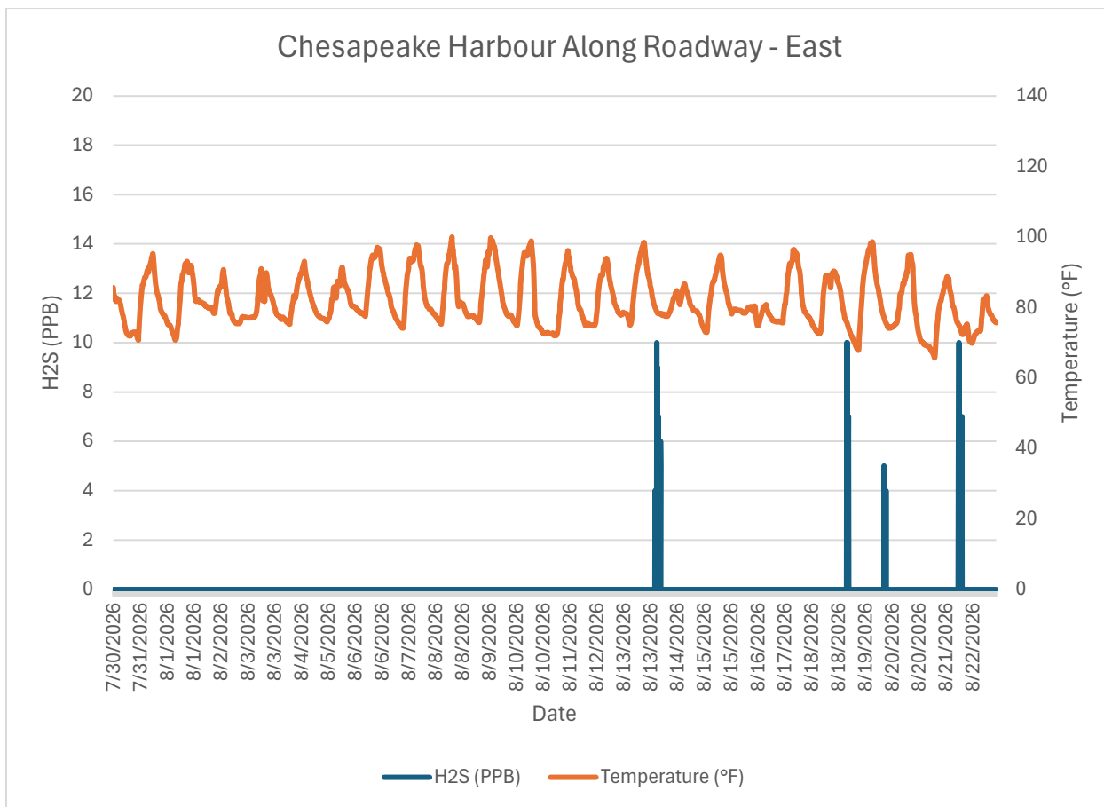
Monitor 5 Neighborhood Chesapeake Harbour Along Roadway - East H2S PPB August, 2026
