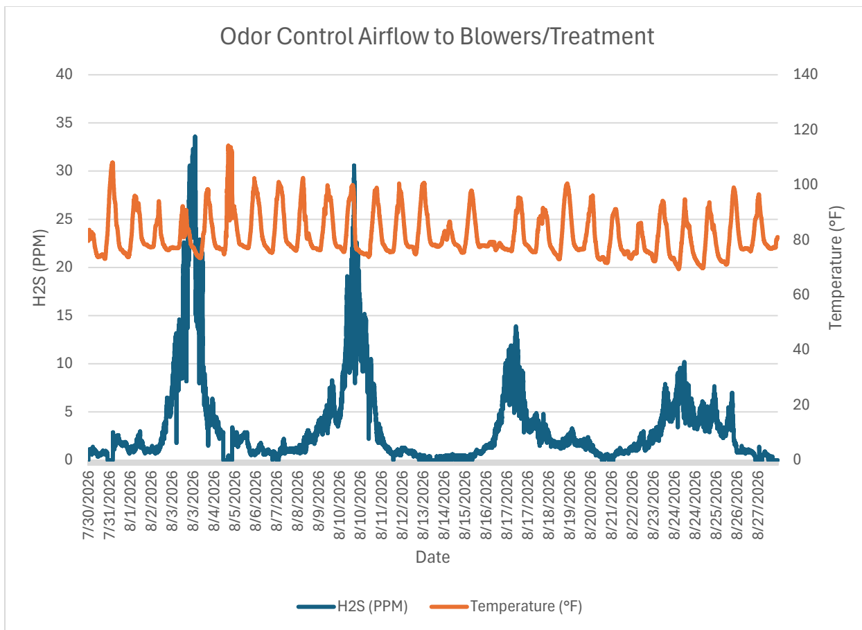
Monitor 3 Within WRF: Odor Control Airflow to Blowers/Treatment H2S PPM August, 2026
