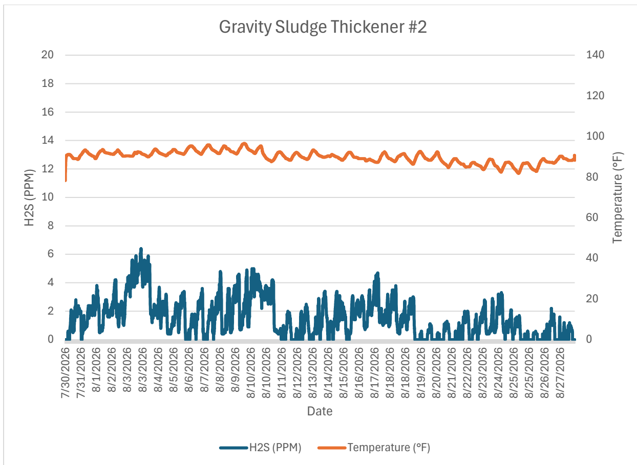
Monitor 4 Within WRF: Gravity Sludge Thickener #2 H2S PPM August, 2026
