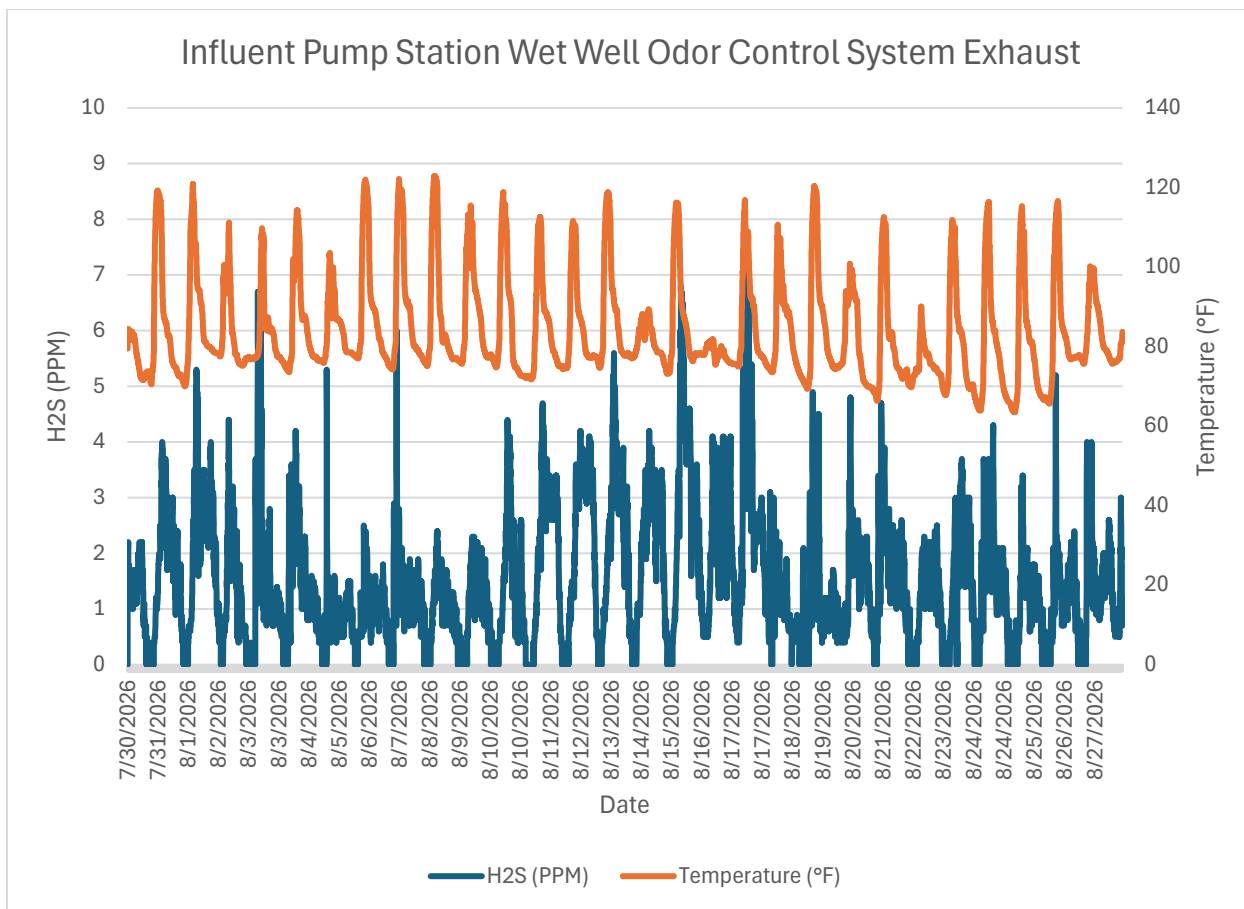
Monitor 1b Within WRF: Influent Pump Station Wet Well Odor Control System Exhaust H2S PPM August, 2026
