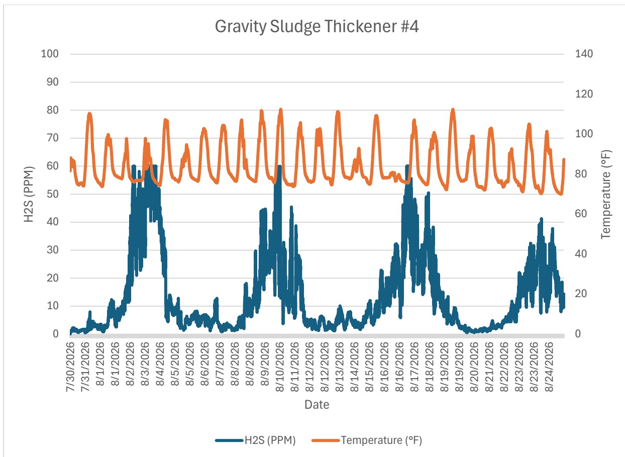
Monitor 5 Within WRF: Gravity Sludge Thickener #4 H2S PPM August, 2026
