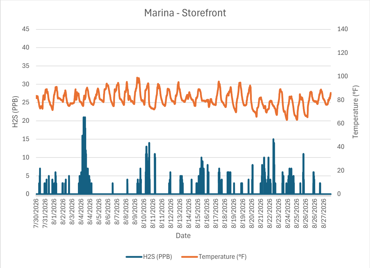
Monitor 1 Neighborhood: Marina – Storefront H2S PPB August, 2026
