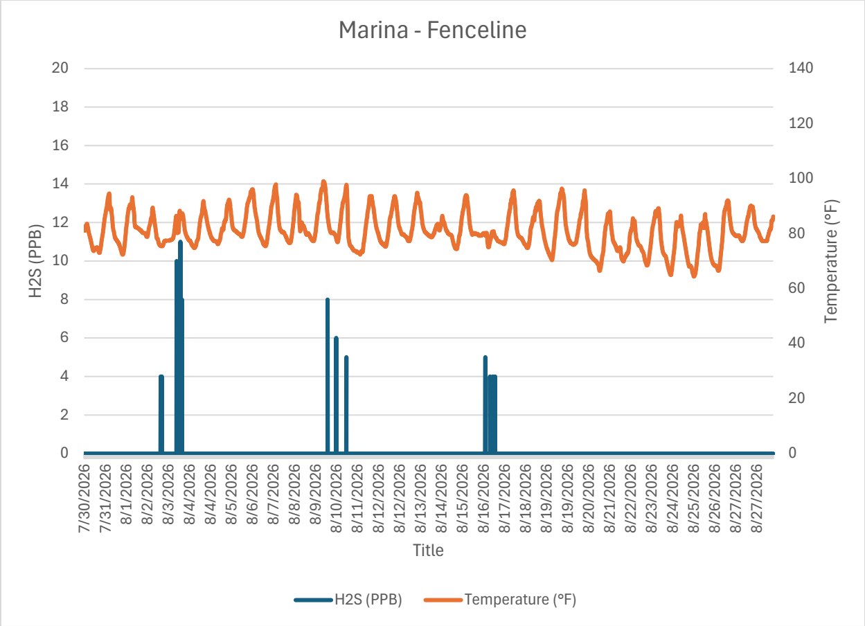
Monitor 2 Neighborhood: Marina – Fenceline H2S PPB August, 2026
