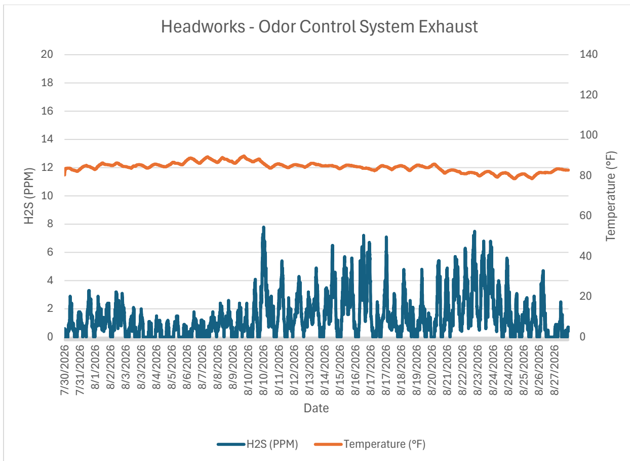
Monitor 2b Within WRF: Headworks – Odor Control System Exhaust H2S PPM August, 2026
