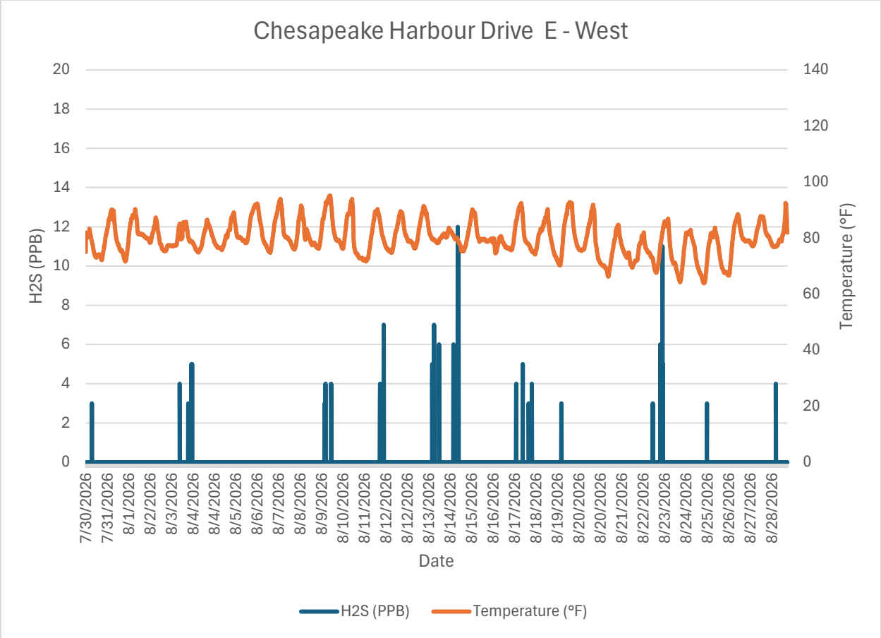
Monitor 6 Neighborhood Chesapeake Harbour Drive E - West H2S PPB August, 2026
