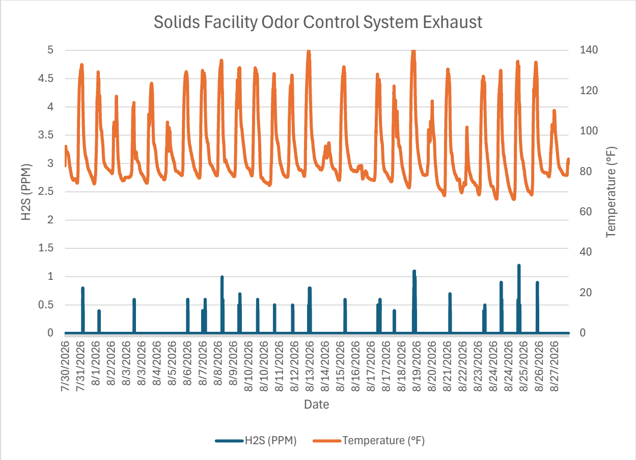
Monitor 6 Within WRF: Solids Facility Odor Control System Exhaust H2S PPM August, 2026
