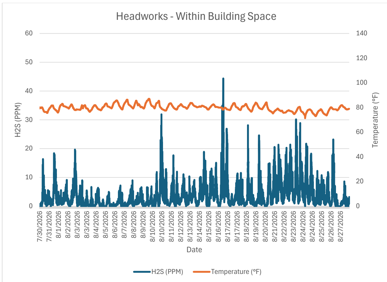
Monitor 2a Within WRF: Headworks – Within Building Space H2S PPM August, 2026
