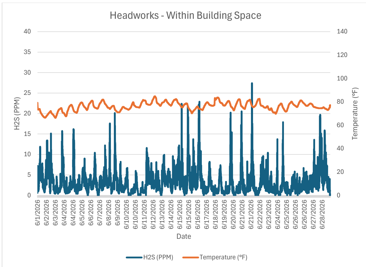
Monitor 2a Within WRF: Headworks – Within Building Space H2S PPM June, 2026
