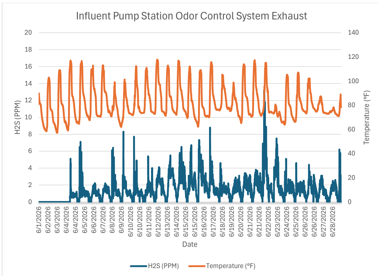
Monitor 1b Within WRF: Influent Pump Station Wet Well Odor Control System Exhaust H2S PPM June, 2026
