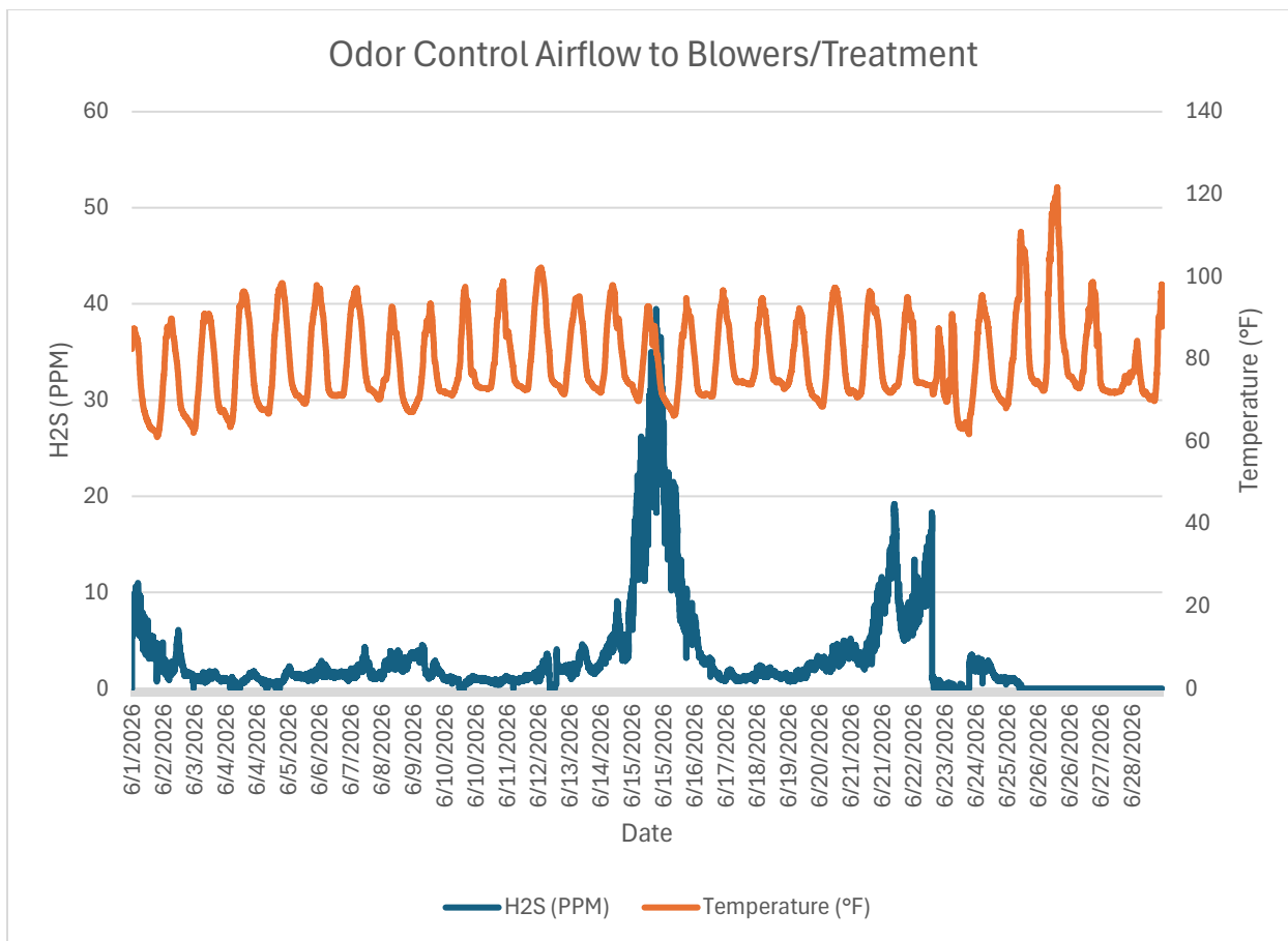
Monitor 3 Within WRF: Odor Control Airflow to Blowers/Treatment H2S PPM June, 2026
