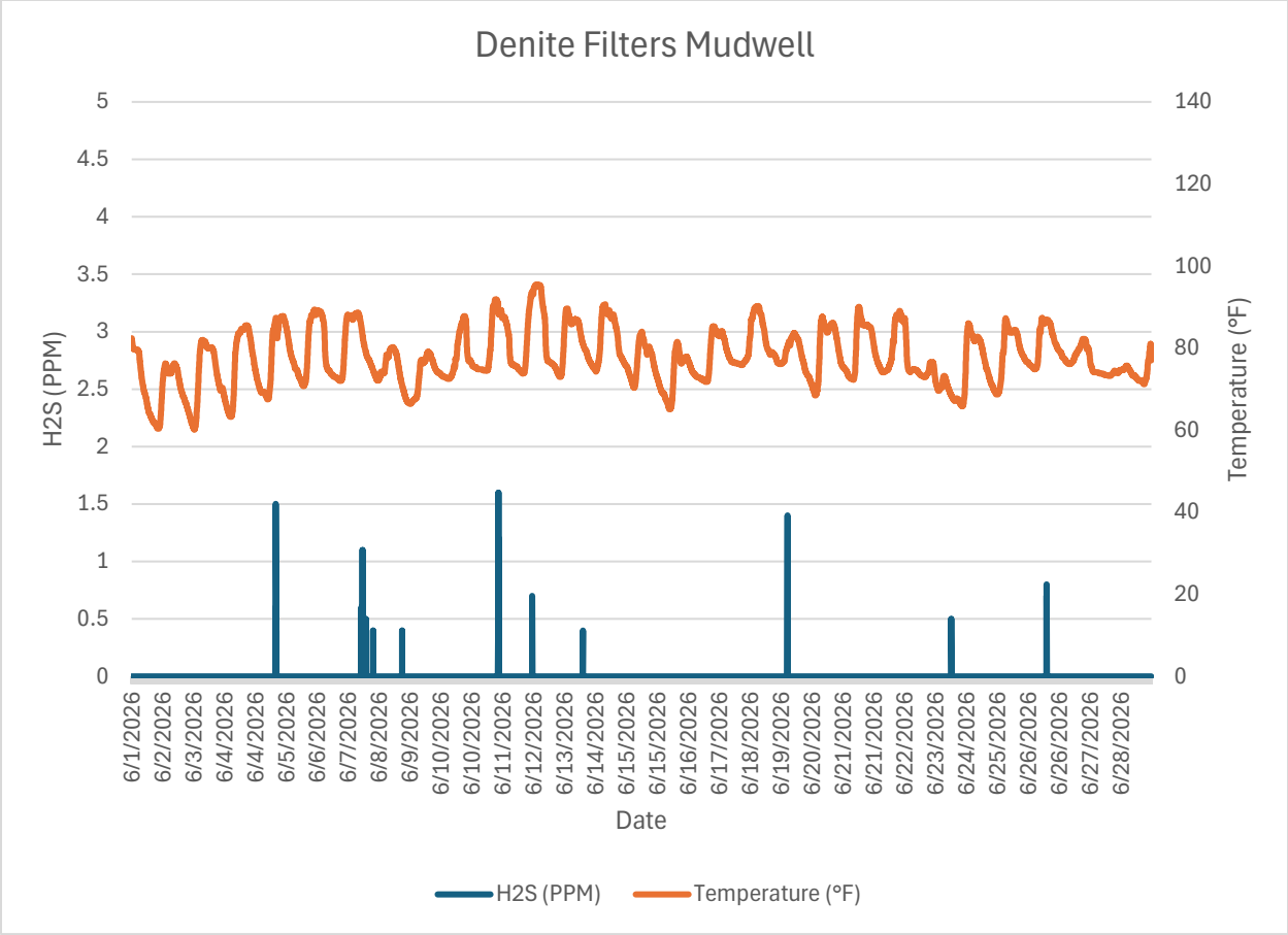
Monitor 7 Within WRF: Denite Filters Mudwell H2S PPM June, 2026
