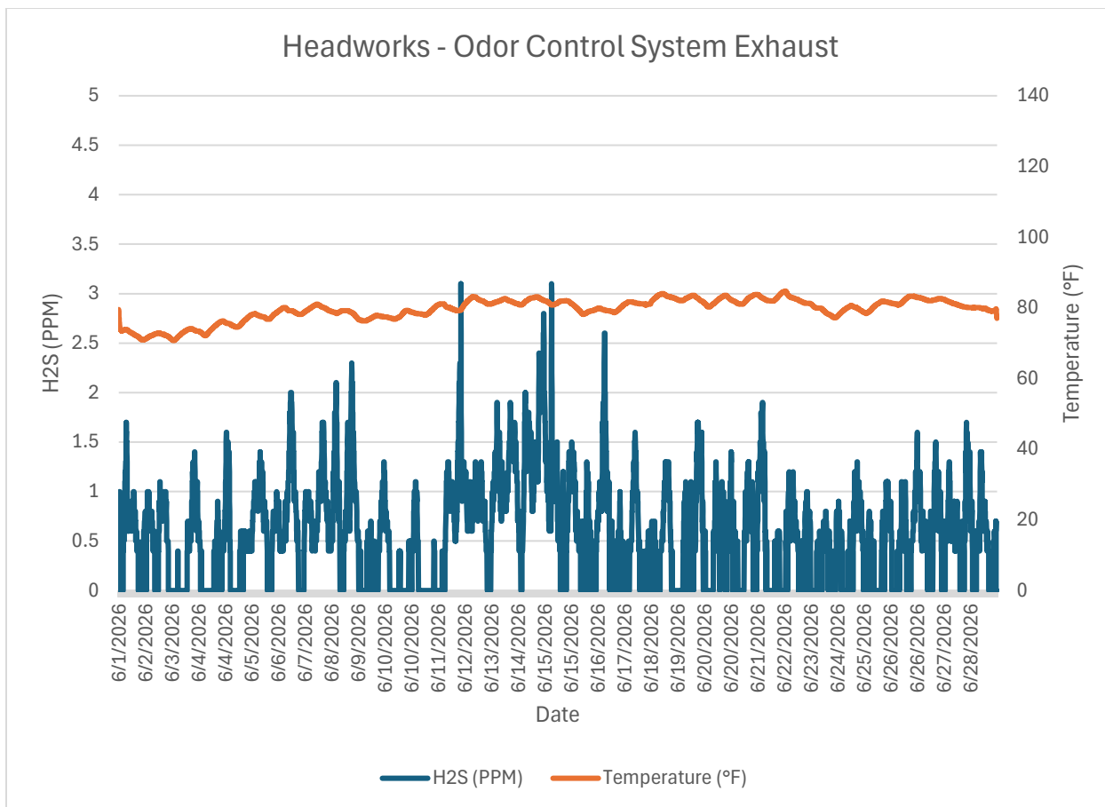
Monitor 2b Within WRF: Headworks – Odor Control System Exhaust H2S PPM June, 2026
