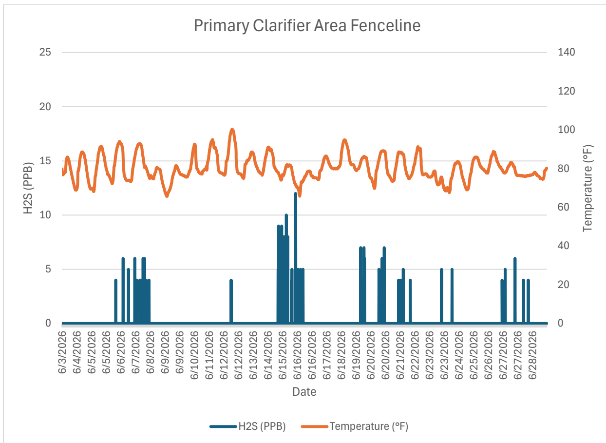
Monitor 2 Fenceline: Primary Clarifier Area Fenceline H2S PPB June, 2026
