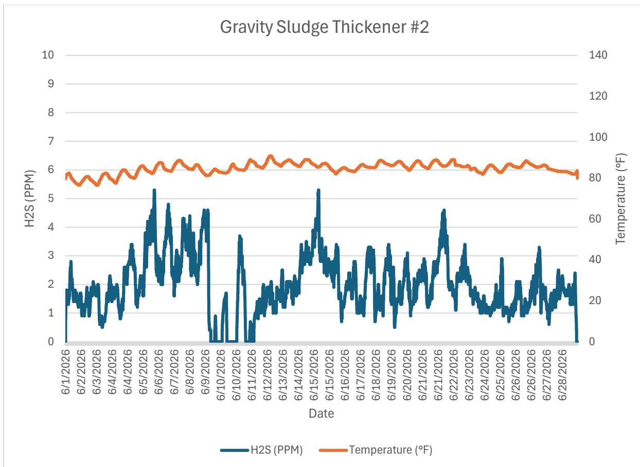
Monitor 4 Within WRF: Gravity Sludge Thickener #2 H2S PPM June, 2026
