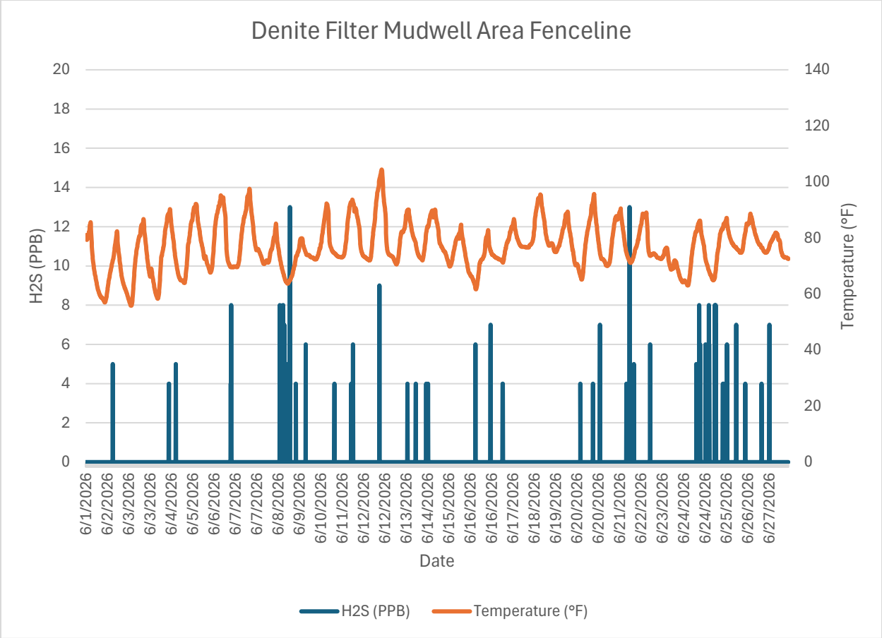
Monitor 3 Fenceline: Denite Filter Mudwell Area Fenceline H2S PPB June, 2026
