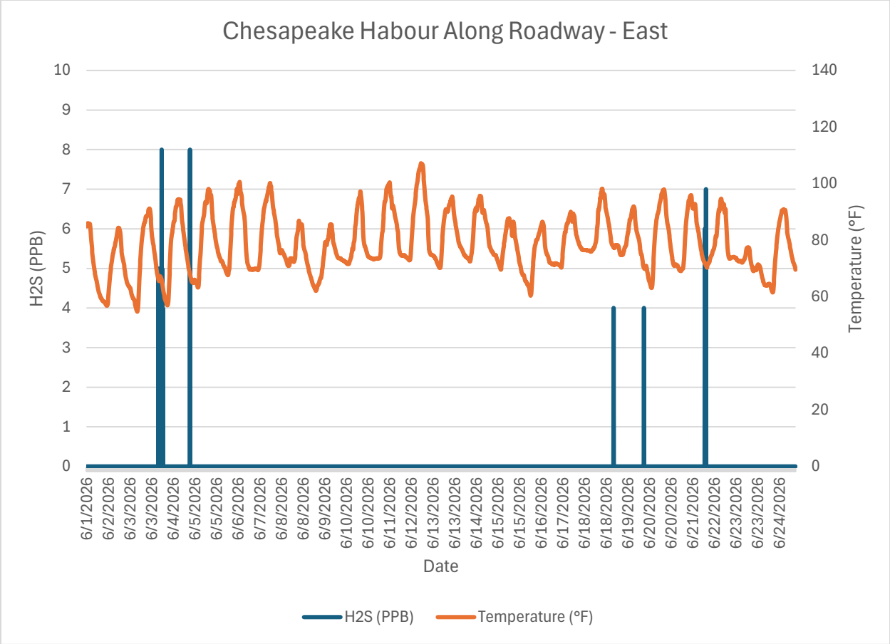
Monitor 5 Neighborhood Chesapeake Harbour Along Roadway - East H2S PPB June, 2026
