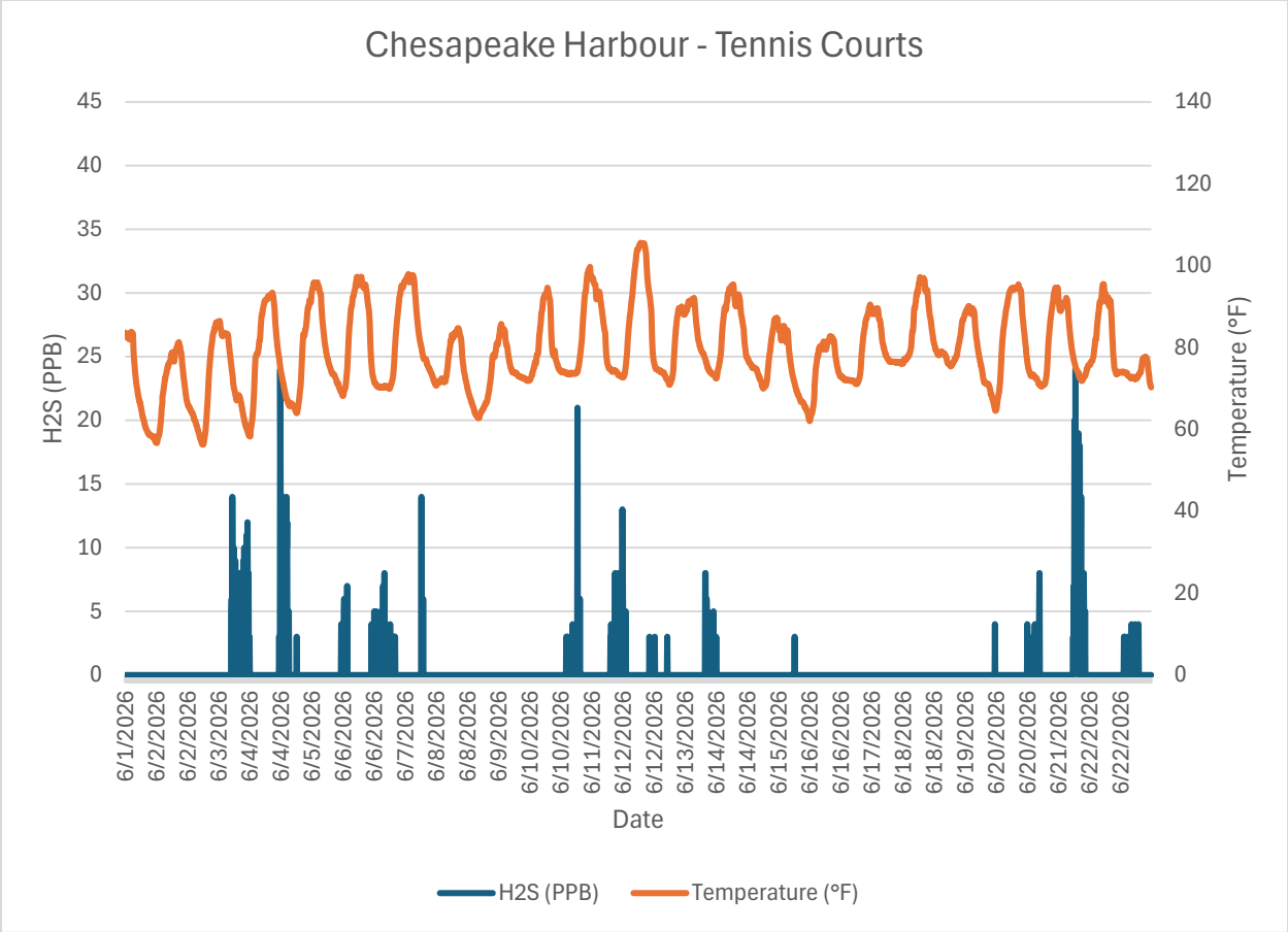
Monitor 4 Neighborhood Chesapeake Harbour – Tennis Courts H2S PPB June, 2026
