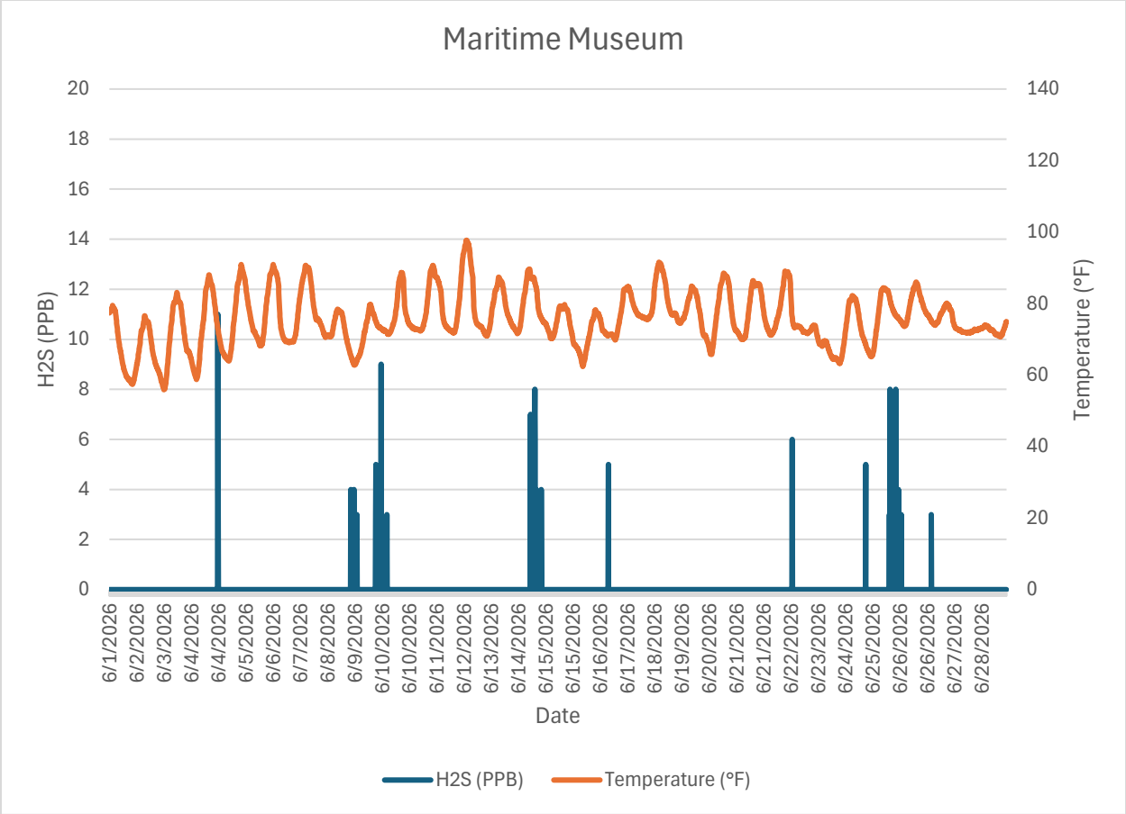
Monitor 3 Neighborhood: Maritime Museum H2S PPB June, 2026
