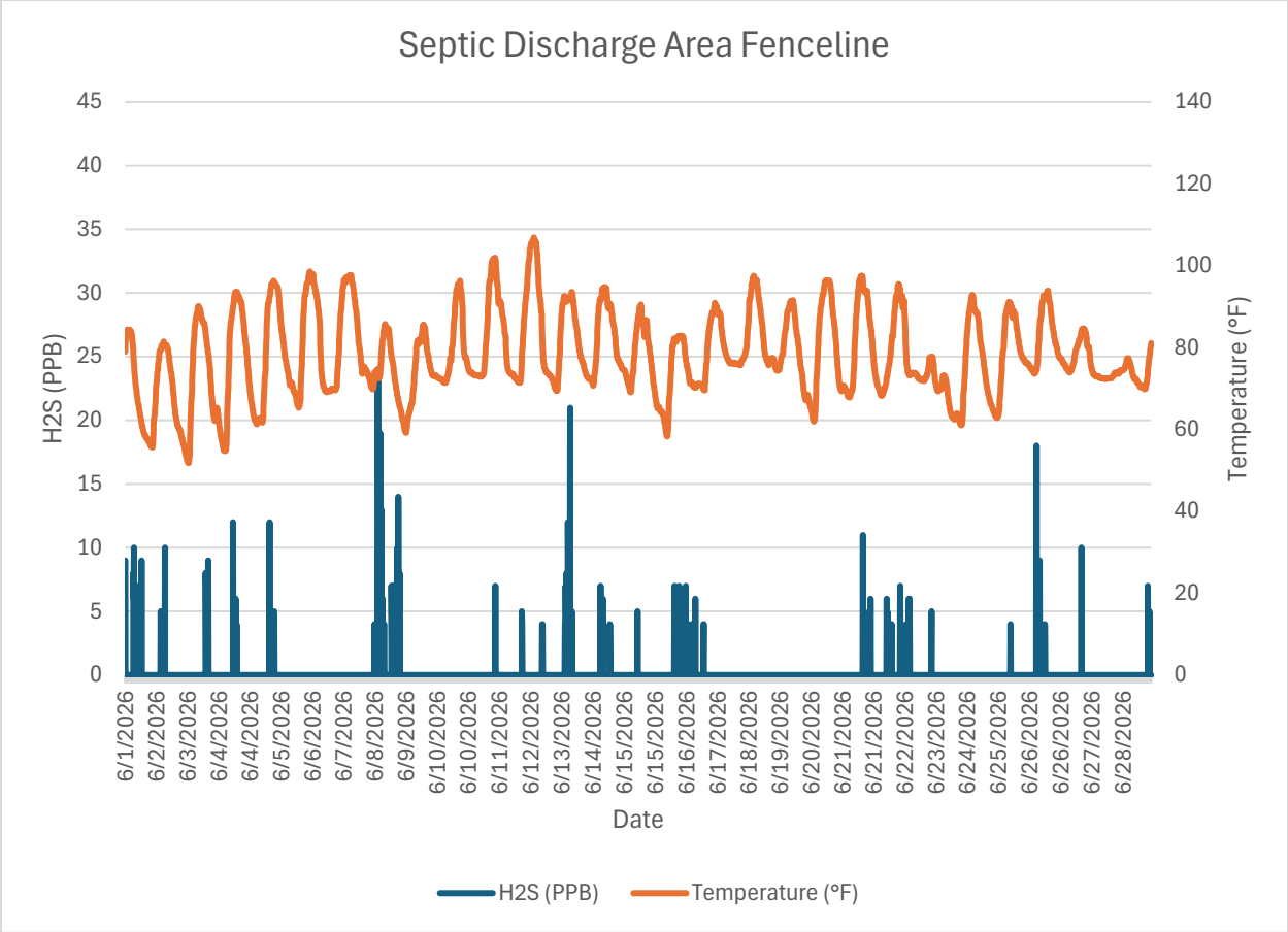
Monitor 1 Fenceline: Septic Hauler Discharge Area Fenceline H2S PPB June, 2026
