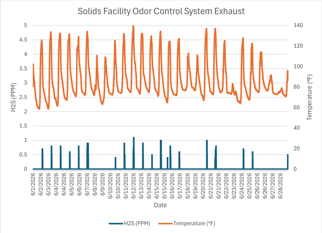
Monitor 6 Within WRF: Solids Facility Odor Control System Exhaust H2S PPM June, 2026
