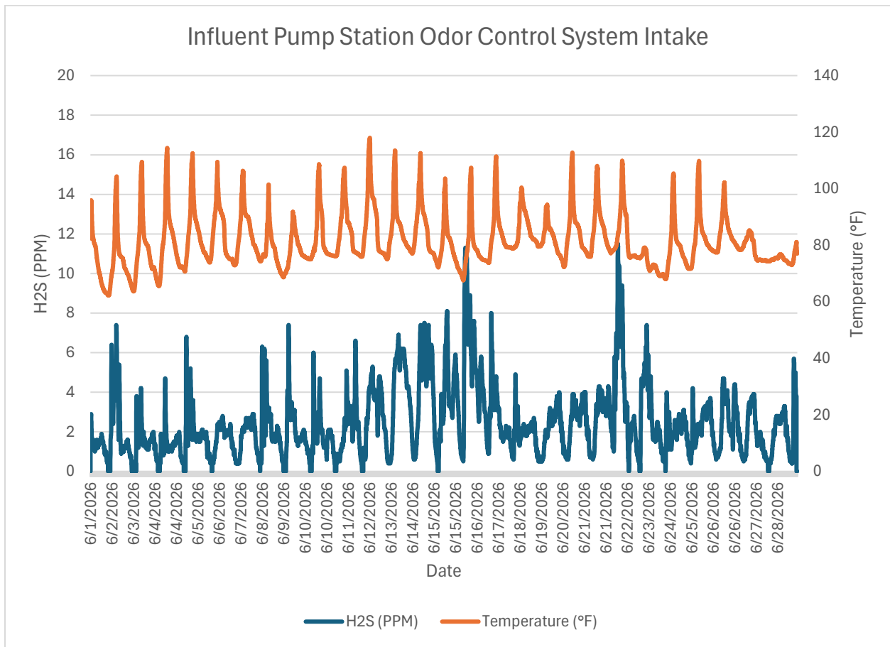
Monitor 1a Within WRF: Influent Pump Station Wet Well Odor Control System Intake H2S PPM June 2026.
