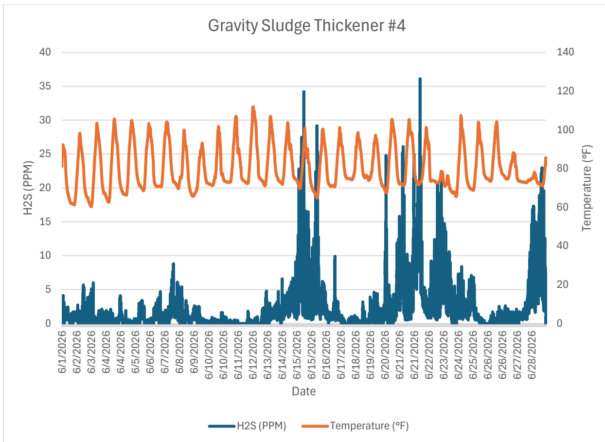
Monitor 5 Within WRF: Gravity Sludge Thickener #4 H2S PPM June, 2026
