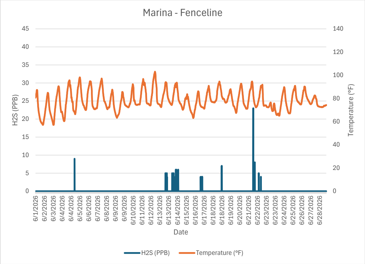
Monitor 2 Neighborhood: Marina – Fenceline H2S PPB June, 2026
