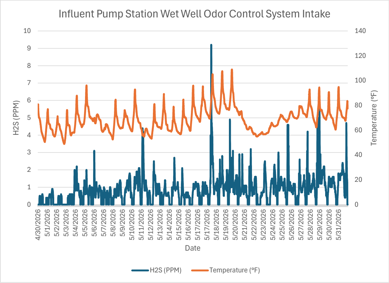
Monitor 1a Within WRF: Influent Pump Station Wet Well Odor Control System Intake H2S PPM May 2026.
