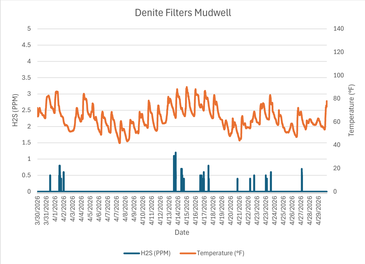
Monitor 7 Within WRF: Denite Filters Mudwell H2S PPM April, 2026
