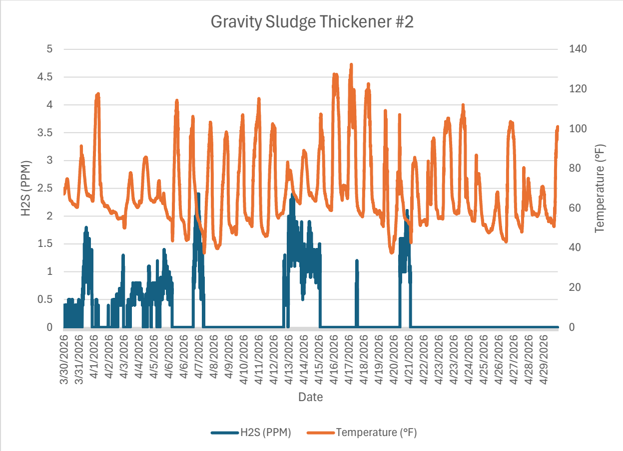
Monitor 4 Within WRF: Gravity Sludge Thickener #2 H2S PPM April, 2026
