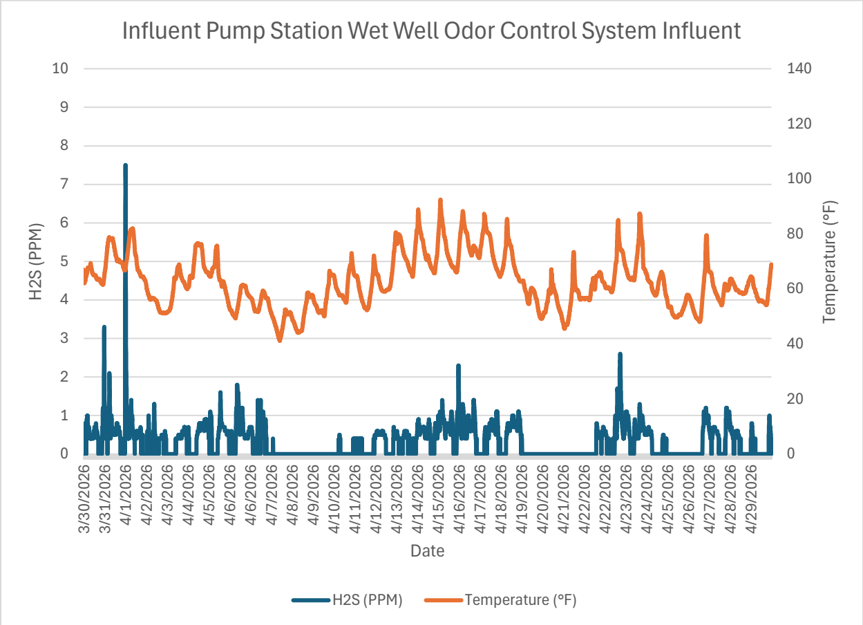
Monitor 1a Within WRF: Influent Pump Station Wet Well Odor Control System Intake H2S PPM April 2026.
