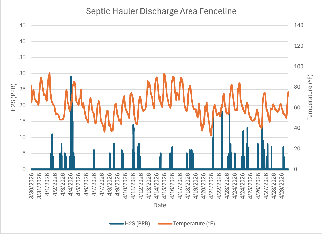
Monitor 1 Fenceline: Septic Hauler Discharge Area Fenceline H2S PPB April, 2026
