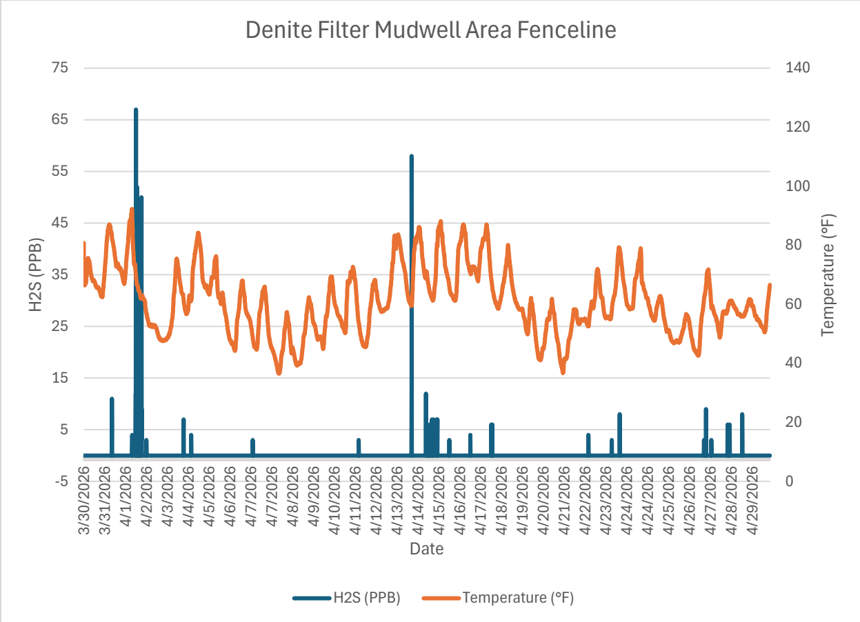
Monitor 3 Fenceline: Denite Filter Mudwell Area Fenceline- North H2S PPB April, 2026
