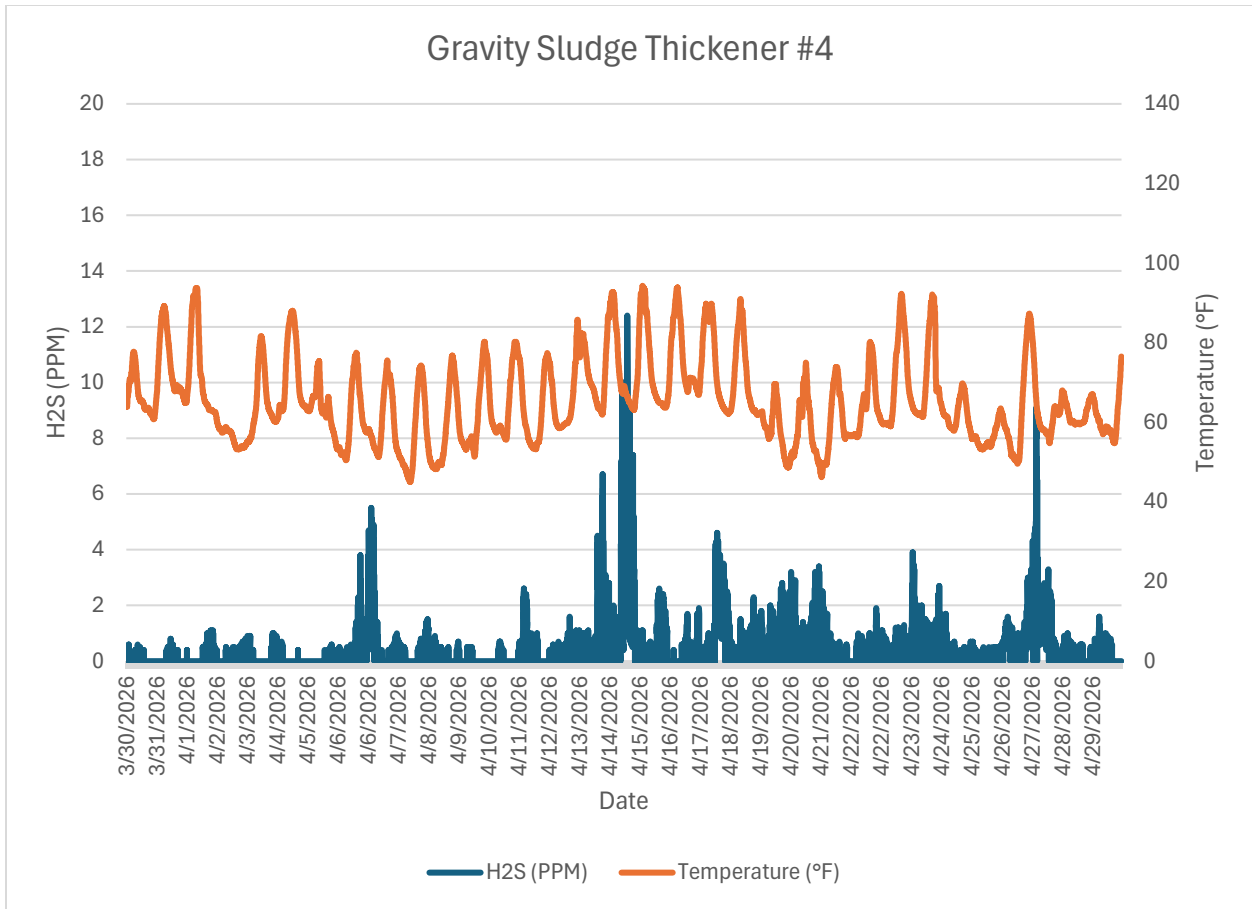
Monitor 5 Within WRF: Gravity Sludge Thickener #4 H2S PPM April, 2026
