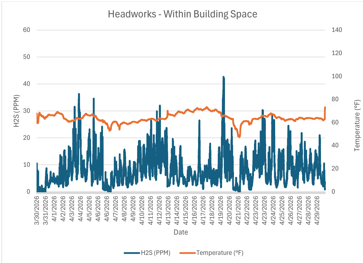
Monitor 2a Within WRF: Headworks – Within Building Space H2S PPM April, 2026
