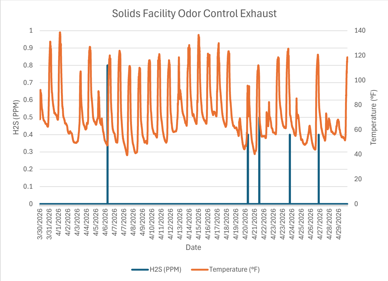
Monitor 6 Within WRF: Solids Facility Odor Control System Exhaust H2S PPM April, 2026
