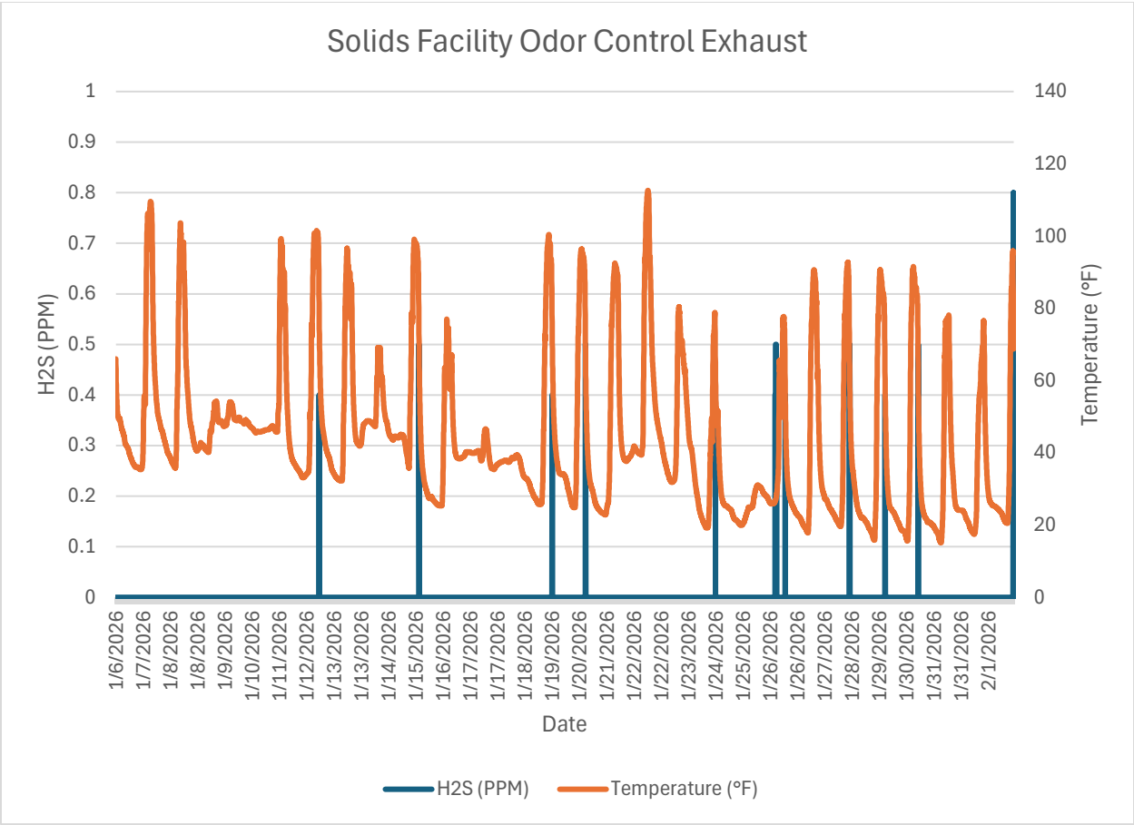
Monitor 6 Within WRF: Solids Facility Odor Control System Exhaust H2S PPM January, 2026
