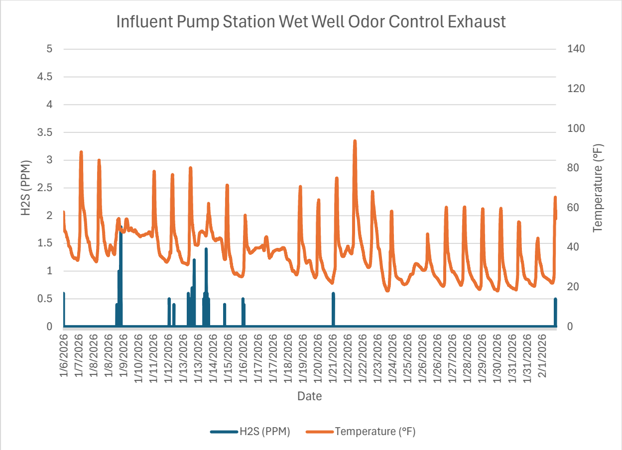
Monitor 1b Within WRF: Influent Pump Station Wet Well Odor Control System Exhaust H2S PPM January, 2026
