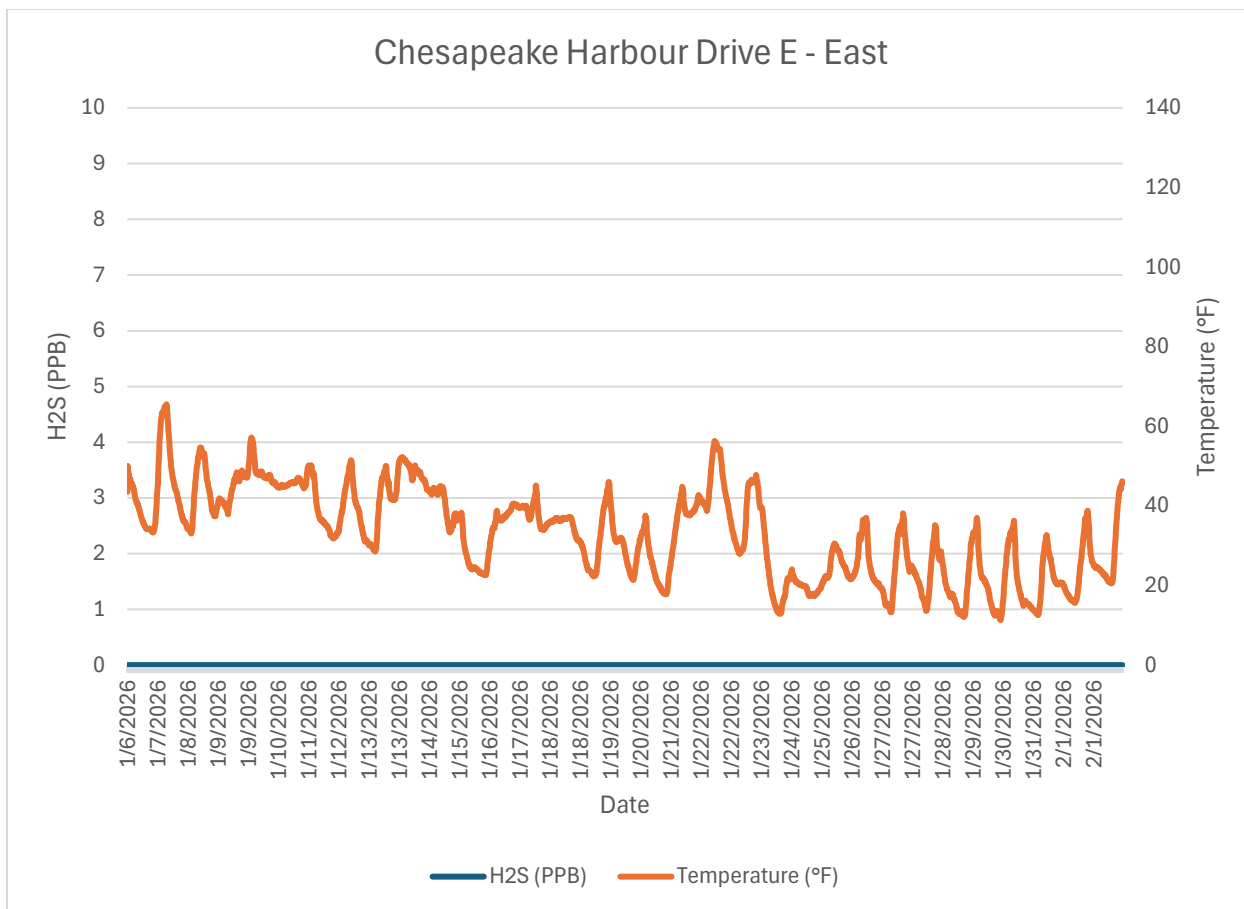
Monitor 7 Neighborhood Chesapeake Harbour Drive E - East (Guard Shack) H2S PPB January, 2026
