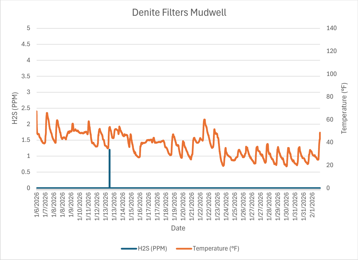
Monitor 7 Within WRF: Denite Filters Mudwell H2S PPM January, 2026
