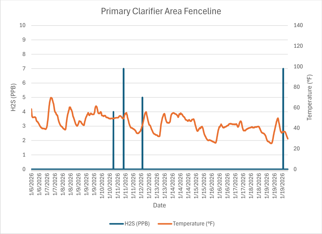
Monitor 2 Fenceline: Primary Clarifier Area Fenceline H2S PPB January, 2026
