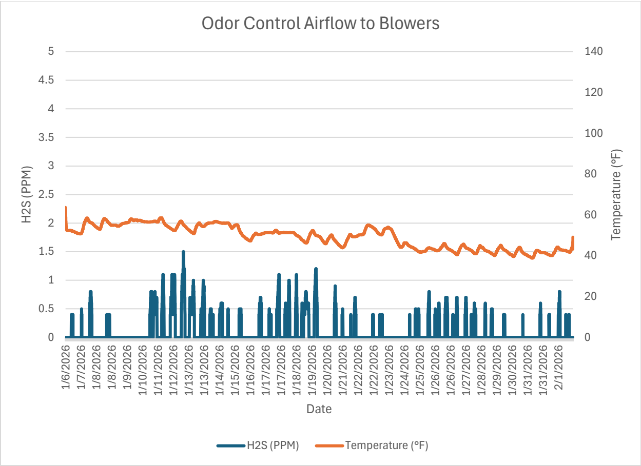
Monitor 4 Within WRF: Odor Control Airflow to Blowers/Treatment H2S PPM January, 2026
