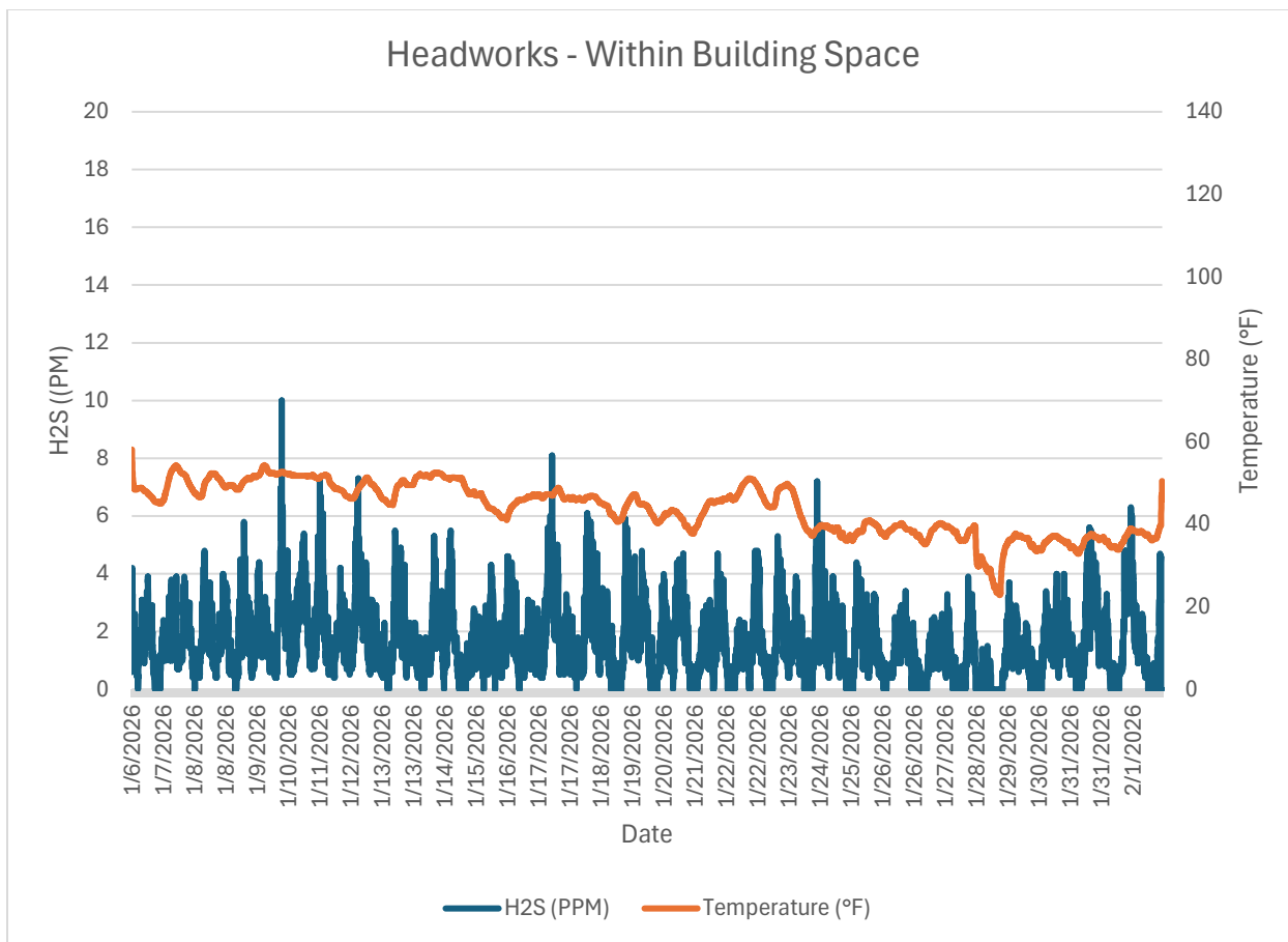
Monitor 2a Within WRF: Headworks – Within Building Space H2S PPM January, 2026
