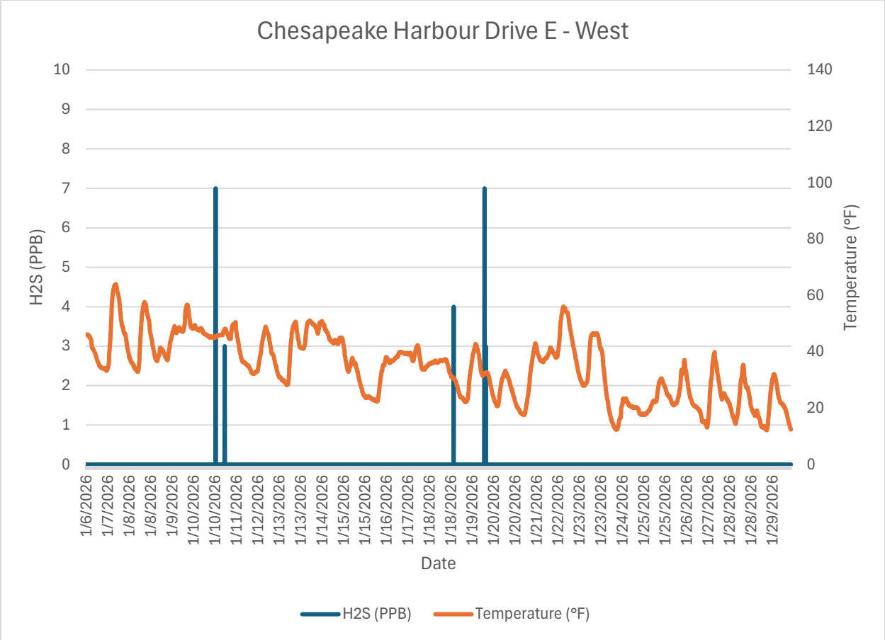
Monitor 6 Neighborhood Chesapeake Harbour Drive E - West H2S PPB January, 2026
