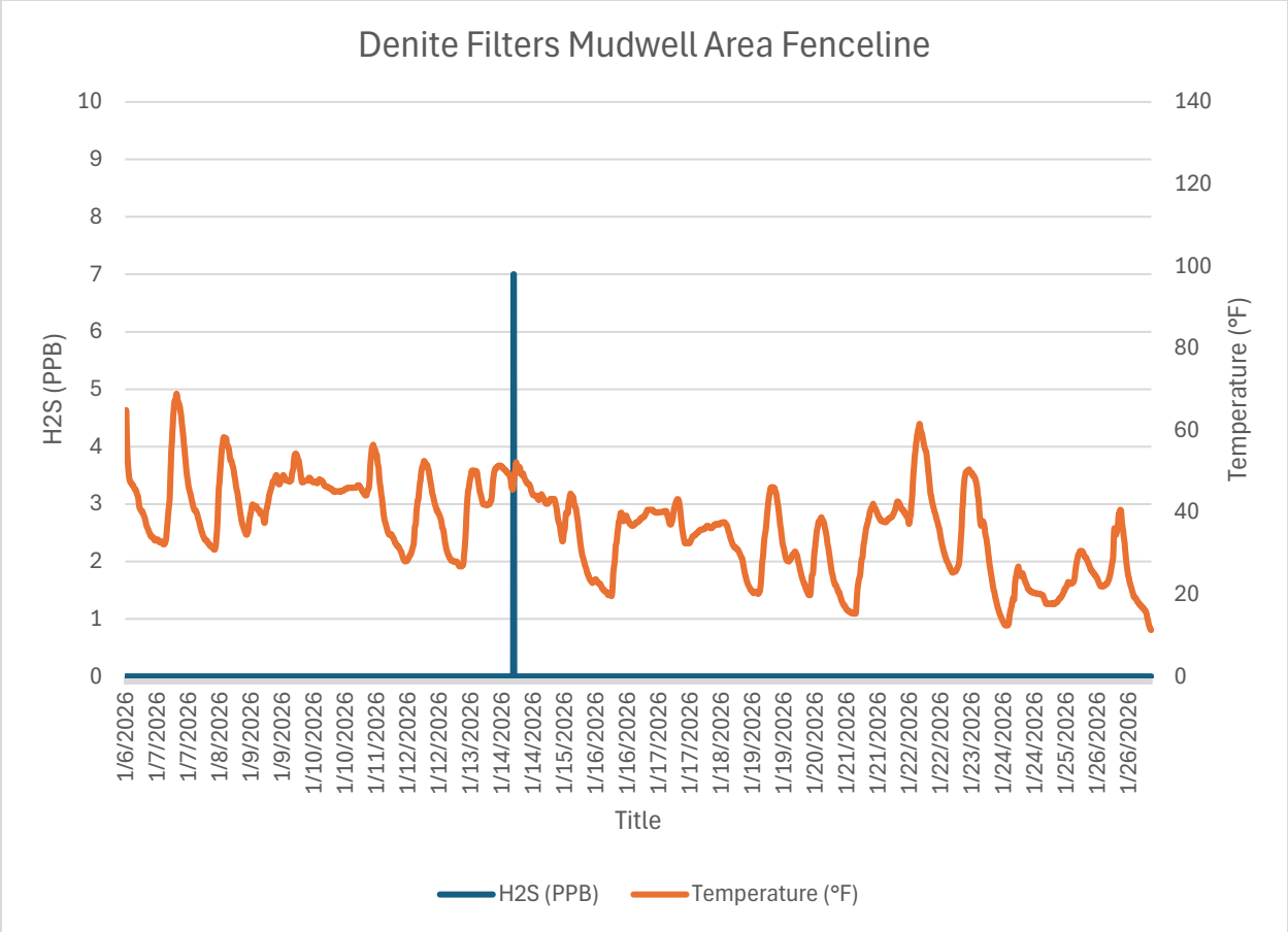
Monitor 3 Fenceline: Denite Filter Mudwell Area Fenceline- North H2S PPB January, 2026
