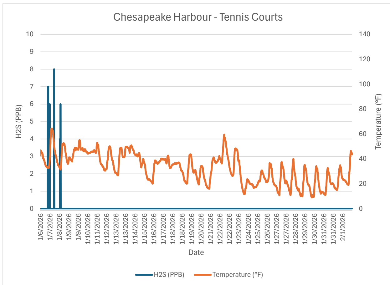
Monitor 4 Neighborhood Chesapeake Harbour – Tennis Courts H2S PPB January, 2026
