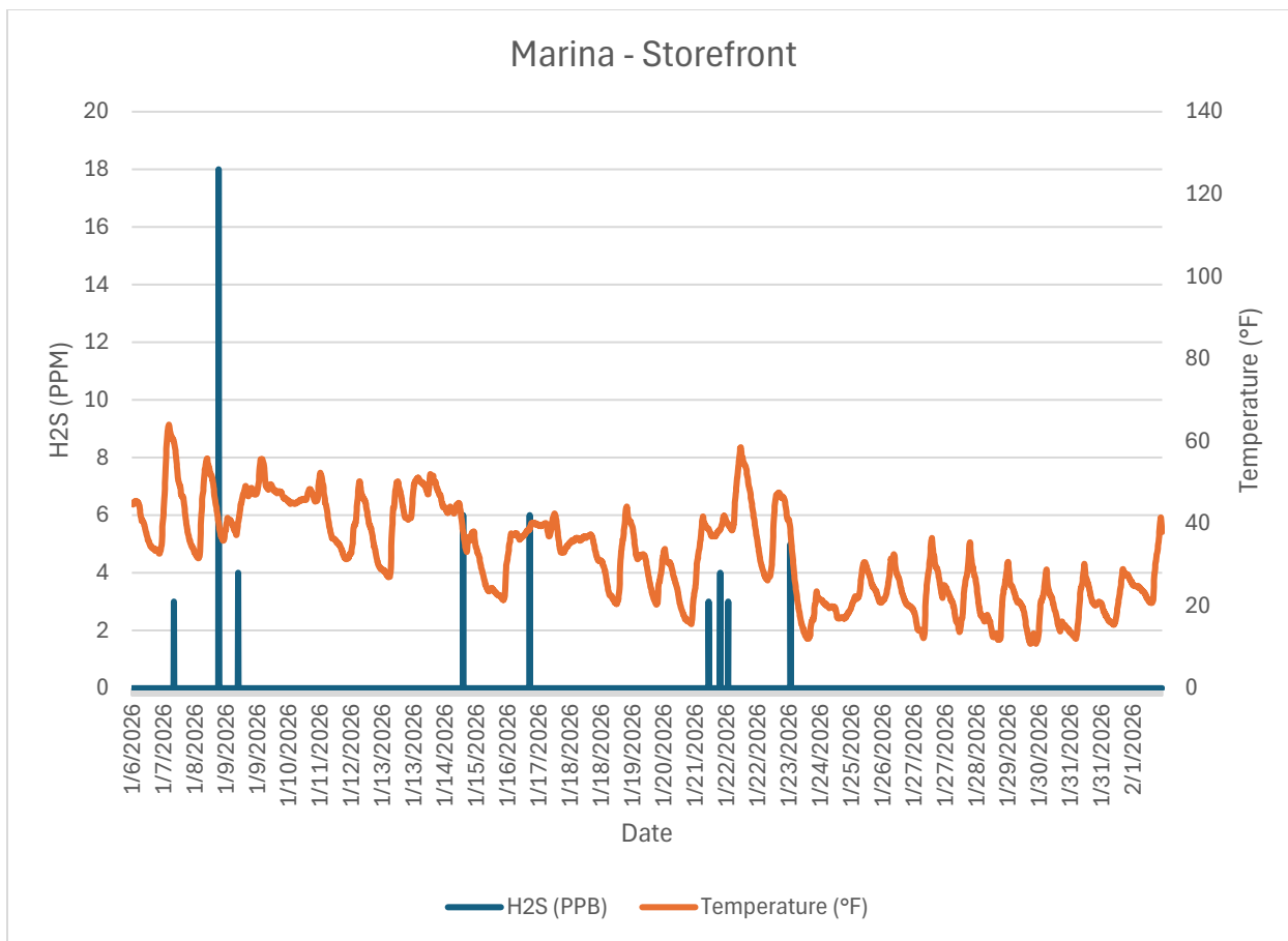
Monitor 1 Neighborhood: Marina – Store Front H2S PPB January, 2026
