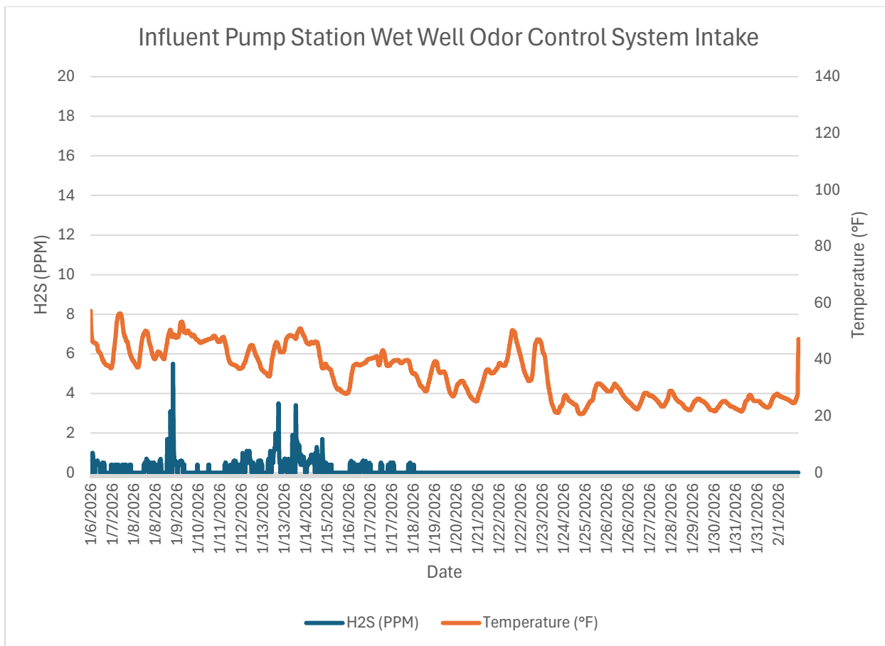
Monitor 1a Within WRF: Influent Pump Station Wet Well Odor Control System Intake H2S PPM January, 2026.
