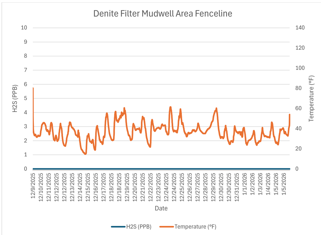
Monitor 3 Fenceline: Denite Filter Mudwell Area Fenceline- North H2S PPB December, 2025
