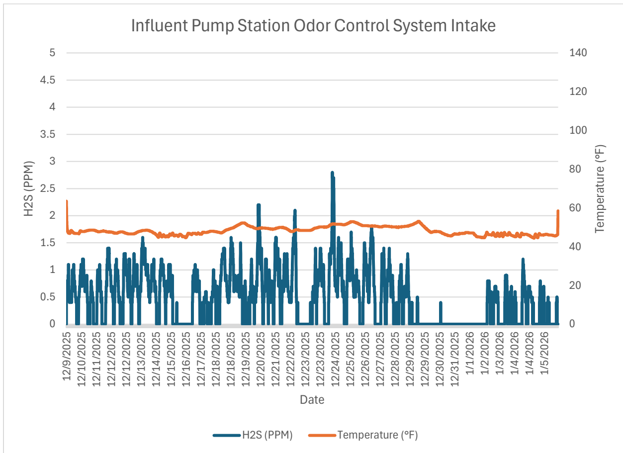
Monitor 1a Within WRF: Influent Pump Station Wet Well Odor Control System Intake H2S PPM December 2025.
