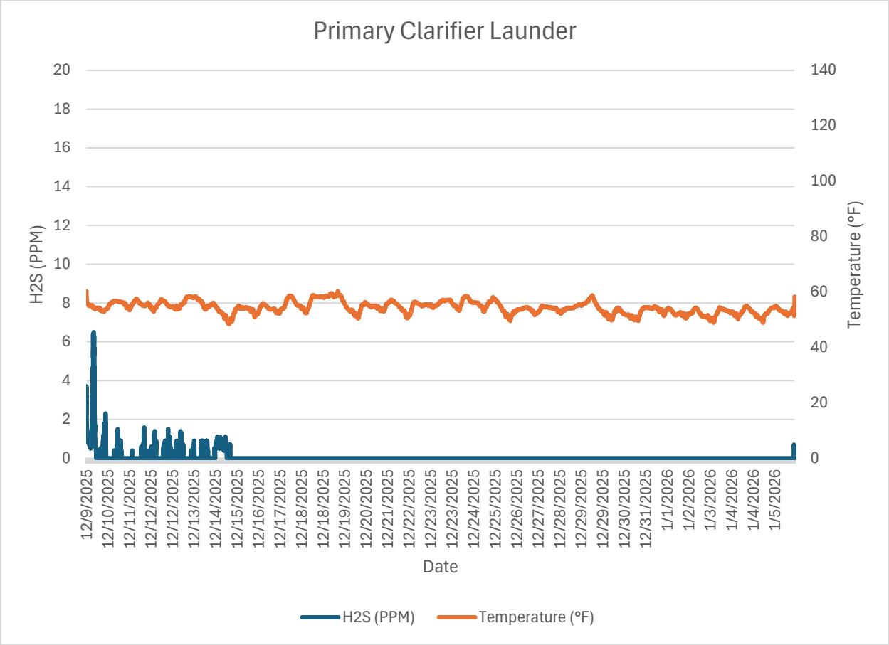
Monitor 3 Within WRF: Primary Clarifier Launder H2S PPM December, 2025
