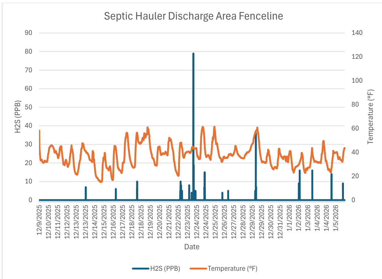
Monitor 1 Fenceline: Septic Hauler Discharge Area Fenceline H2S PPB December, 2025
