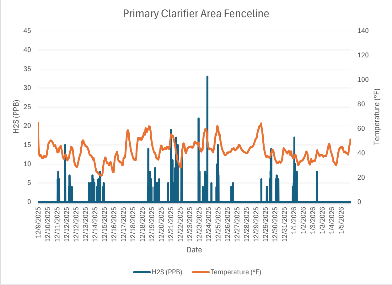
Monitor 2 Fenceline: Primary Clarifier Area Fenceline H2S PPB December, 2025
