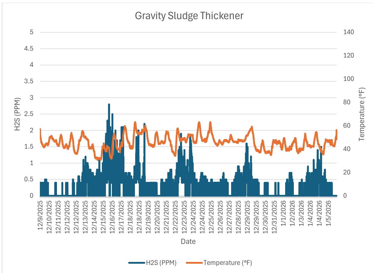
Monitor 5 Within WRF: Gravity Sludge Thickener H2S PPM December, 2025
