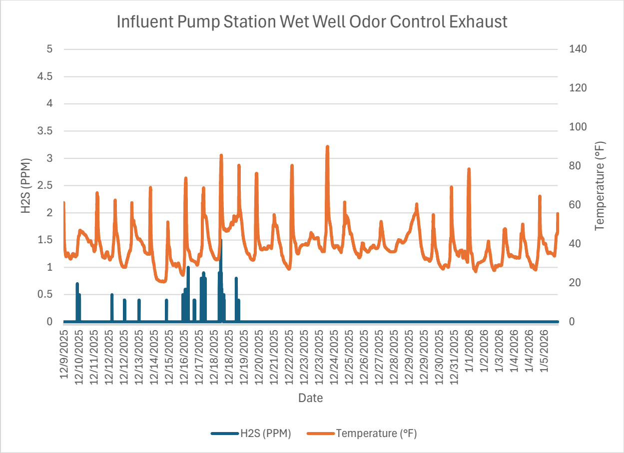
Monitor 1b Within WRF: Influent Pump Station Wet Well Odor Control System Exhaust H2S PPM December, 2025
