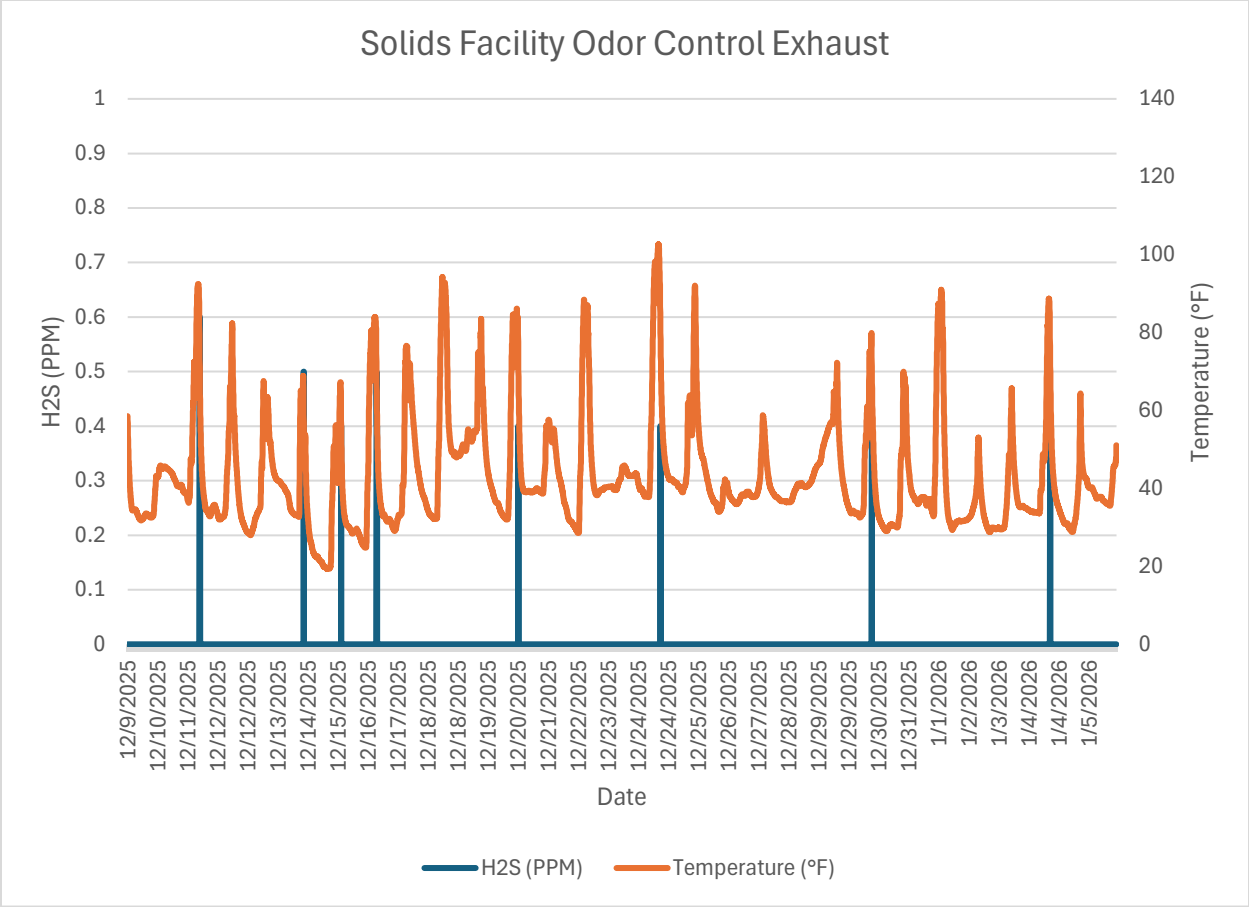
Monitor 6 Within WRF: Solids Facility Odor Control System Exhaust H2S PPM December, 2025
