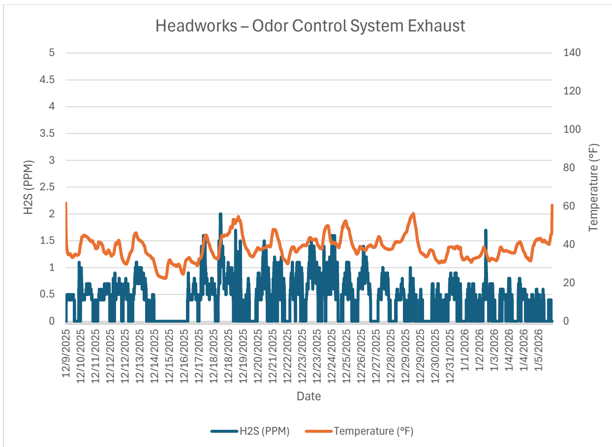
Monitor 2b Within WRF: Headworks – Odor Control System Exhaust H2S PPM December, 2025
