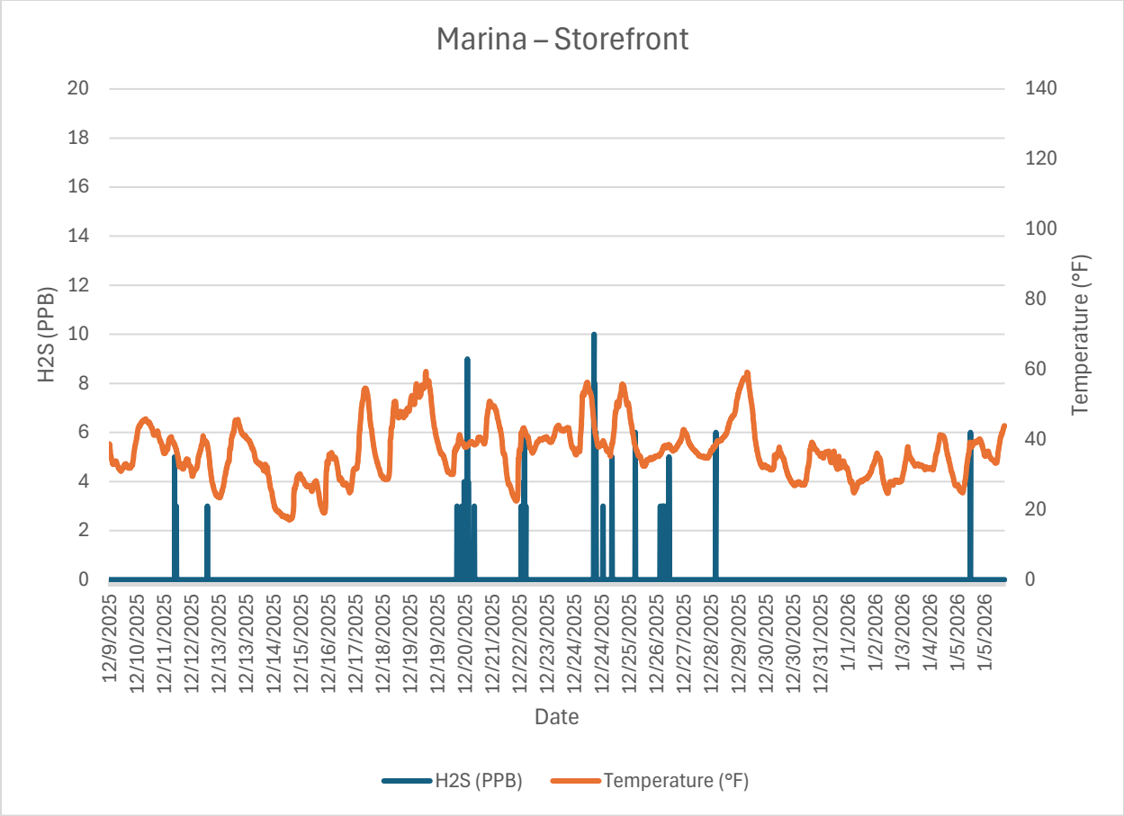
Monitor 1 Neighborhood: Marina – Store Front H2S PPB December, 2025
