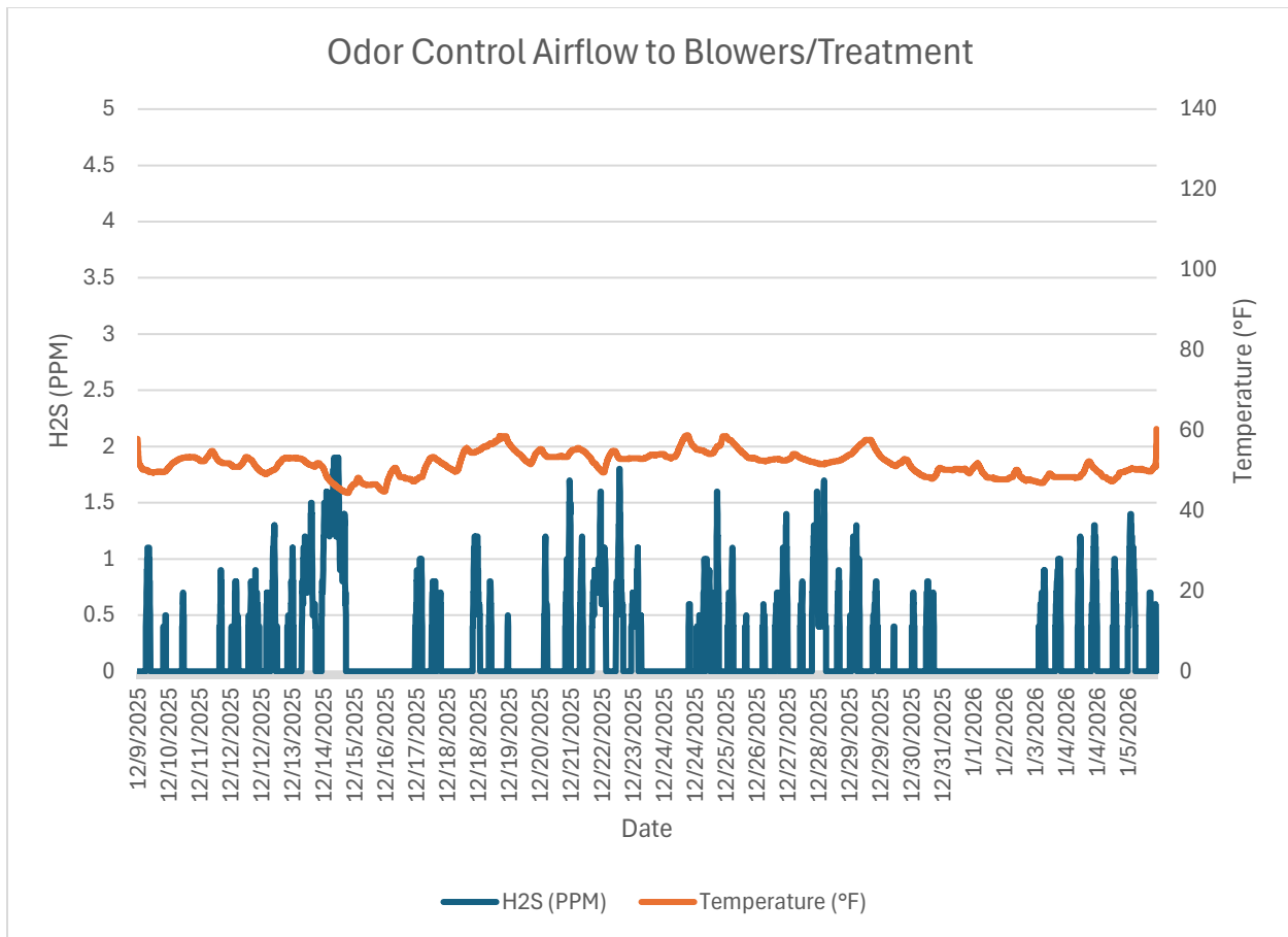
Monitor 4 Within WRF: Odor Control Airflow to Blowers/Treatment H2S PPM December, 2025
