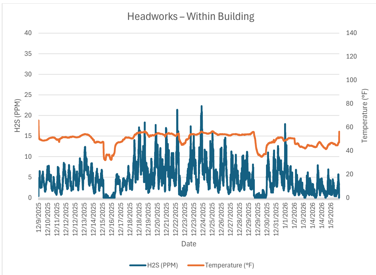
Monitor 2a Within WRF: Headworks – Within Building Space H2S PPM December, 2025
