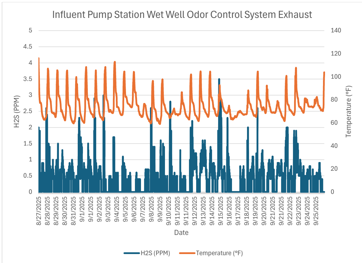
Monitor 1b Within WRF: Influent Pump Station Wet Well Odor Control System Exhaust H2S PPM September, 2025
