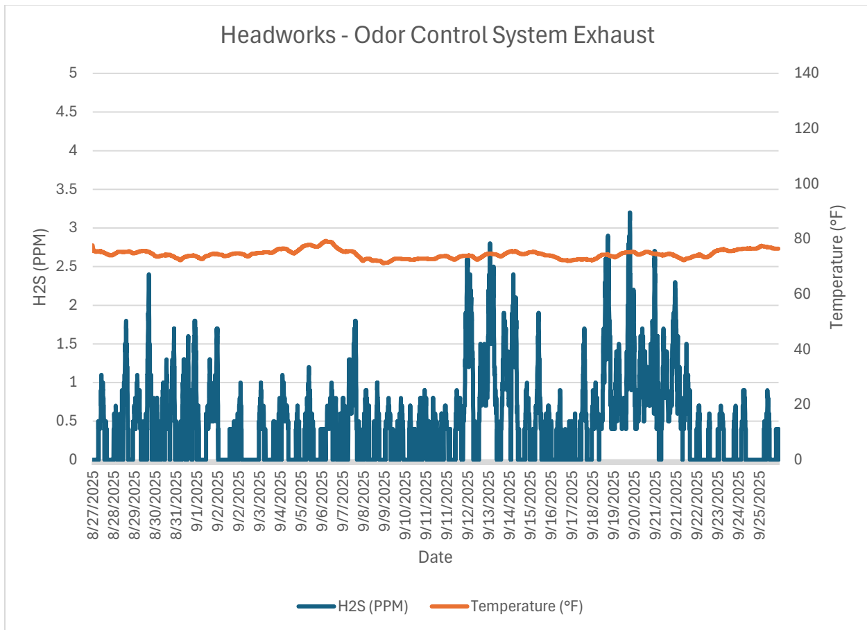
Monitor 2b Within WRF: Headworks Odor Control System Exhaust H2S PPM September, 2025
