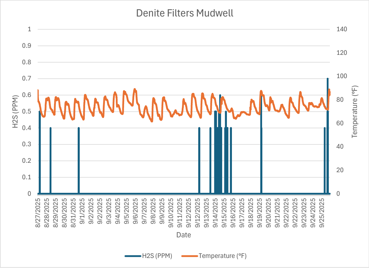
Monitor 7 Within WRF: Denite Filters Mudwell H2S PPM September, 2025
