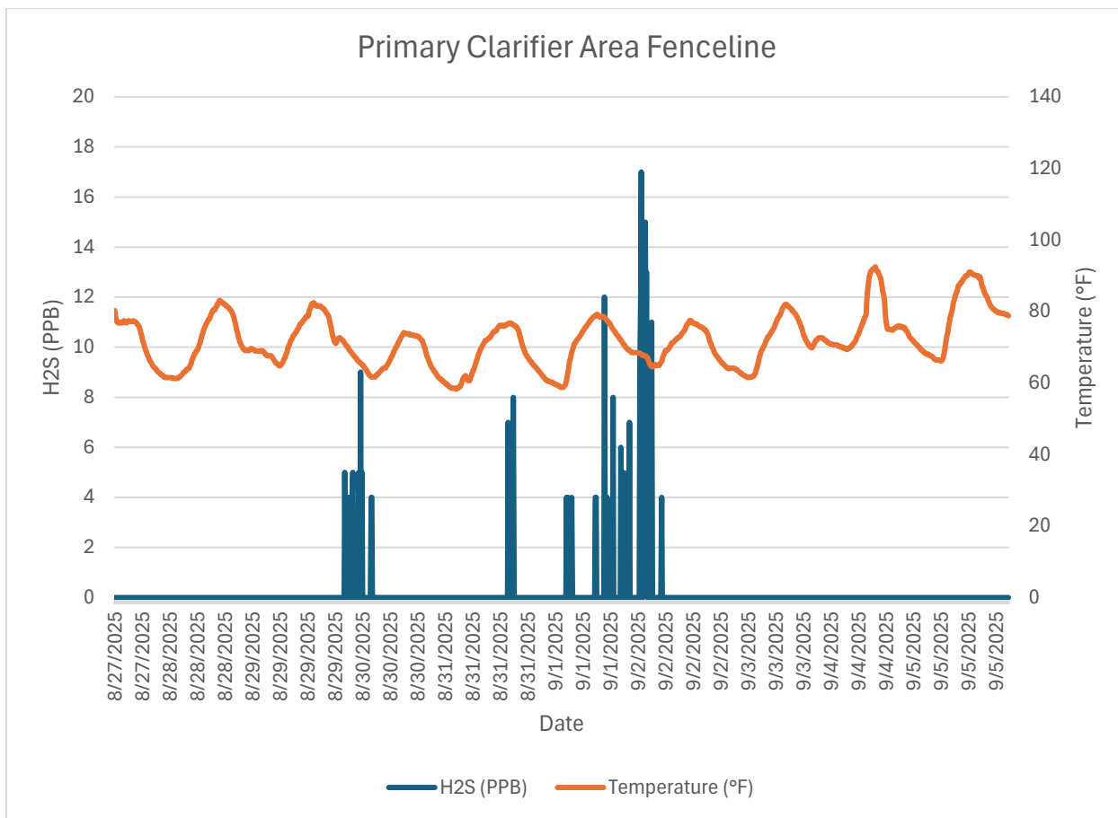
Monitor 2 Fenceline: Primary Clarifier Area Fenceline H2S PPB September, 2025
