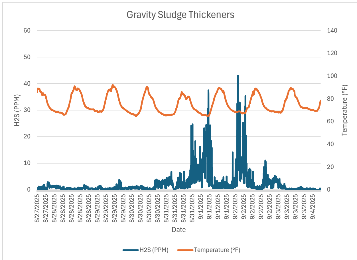
Monitor 5 Within WRF: Gravity Sludge Thickener H2S PPM September, 2025 Monitor was taken OOS on 9/4/25 for calibration.
