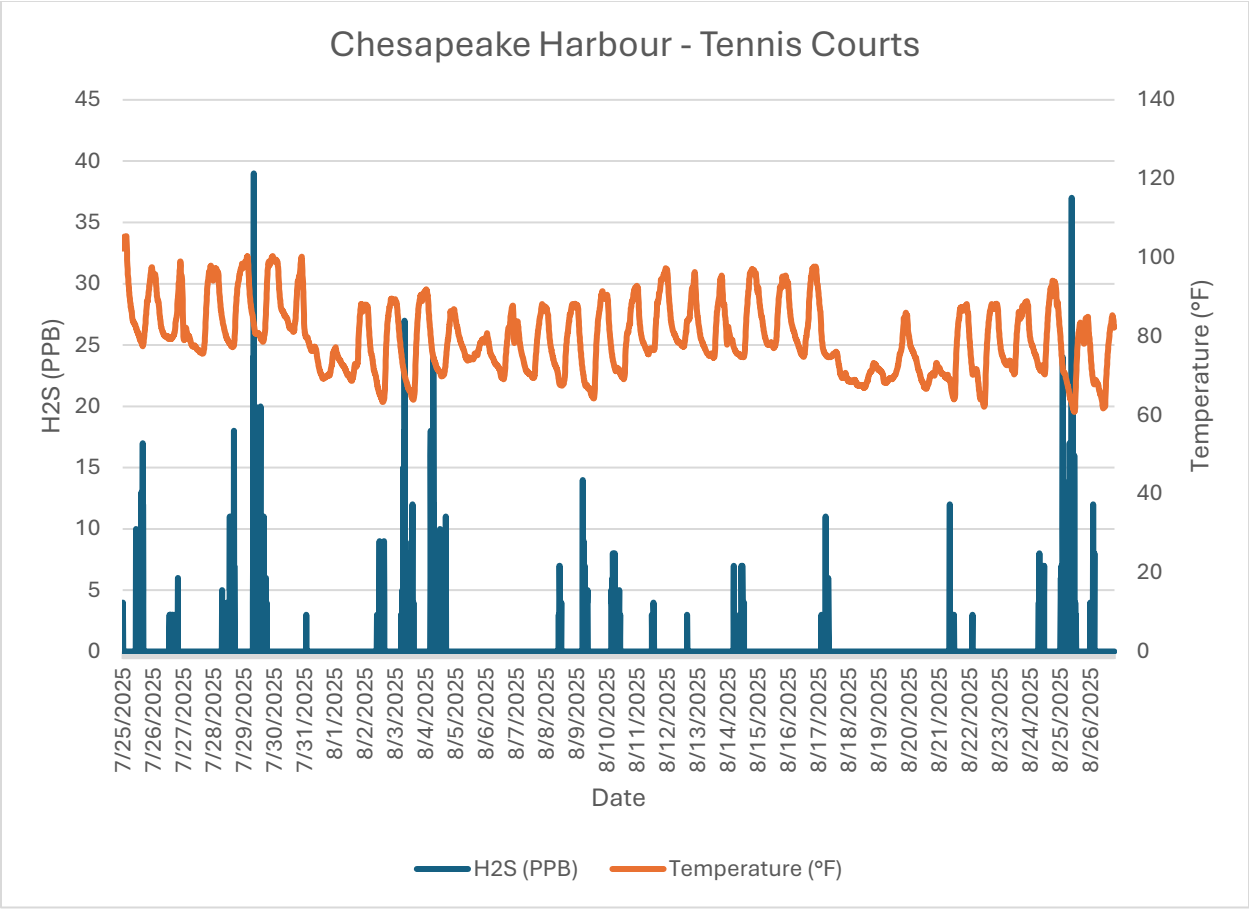
Monitor 4 Neighborhood Chesapeake Harbour – Tennis Courts H2S PPB August, 2025
