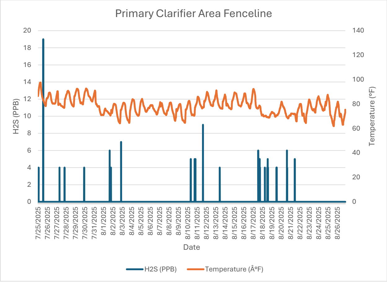
Monitor 2 Fenceline: Primary Clarifier Area Fenceline H2S PPB August, 2025
