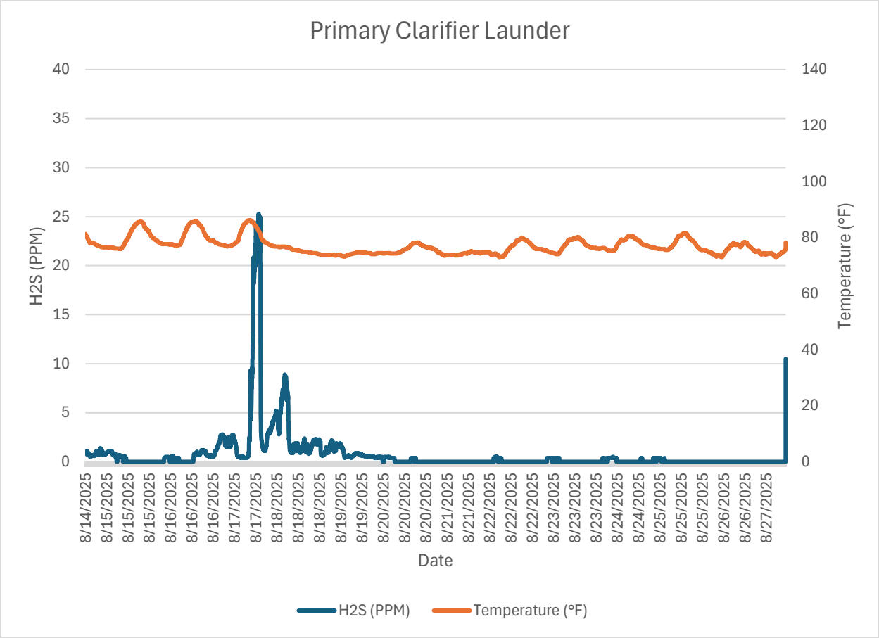
Monitor 3 Within WRF: Primary Clarifier Launder H2S PPM August, 2025
