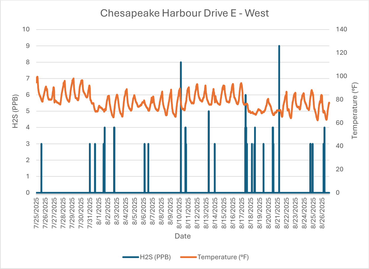
Monitor 6 Neighborhood Chesapeake Harbour Drive E - West H2S PPB August, 2025
