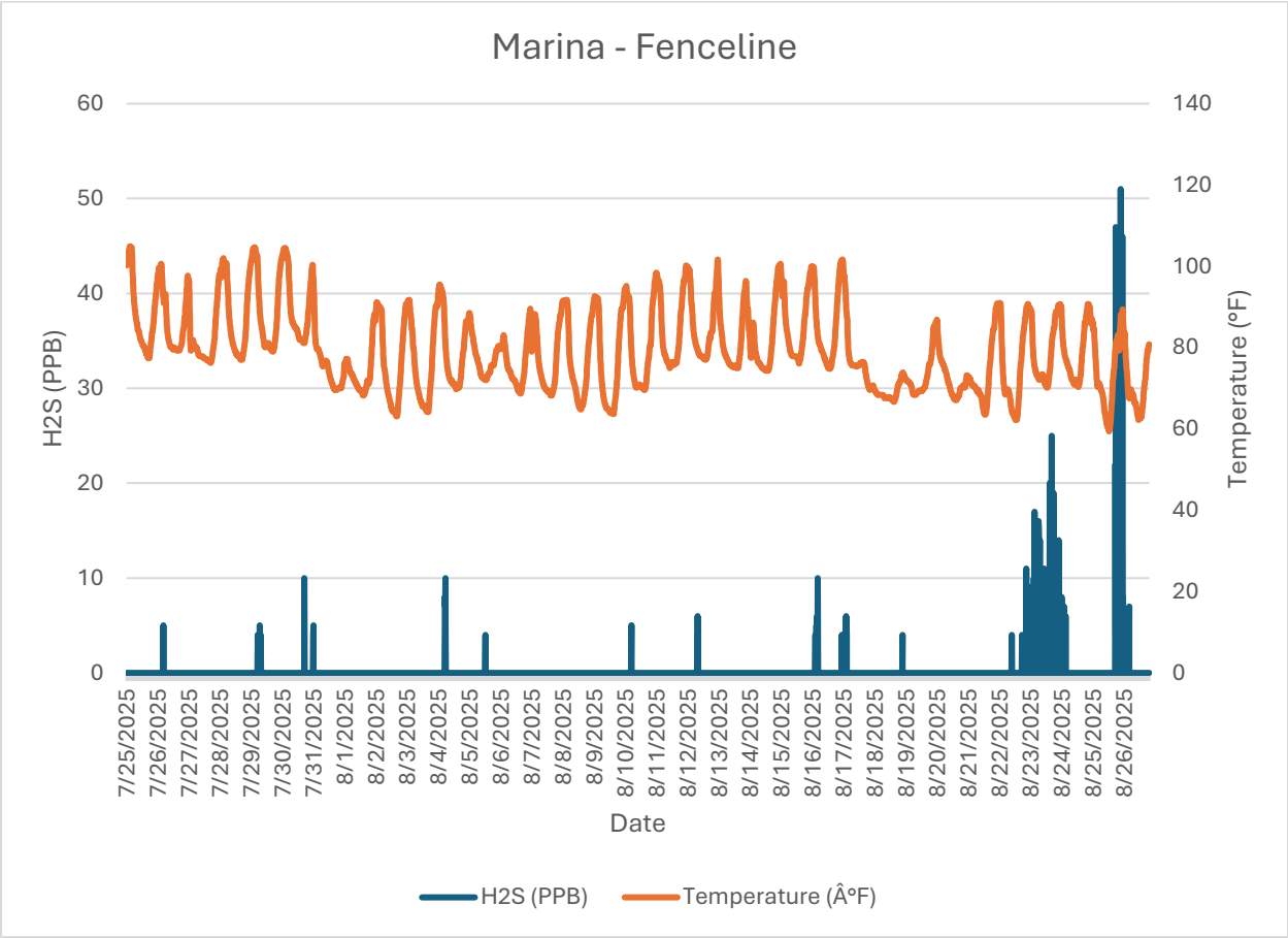
Monitor 2 Neighborhood: Marina – Fenceline H2S PPB August, 2025
