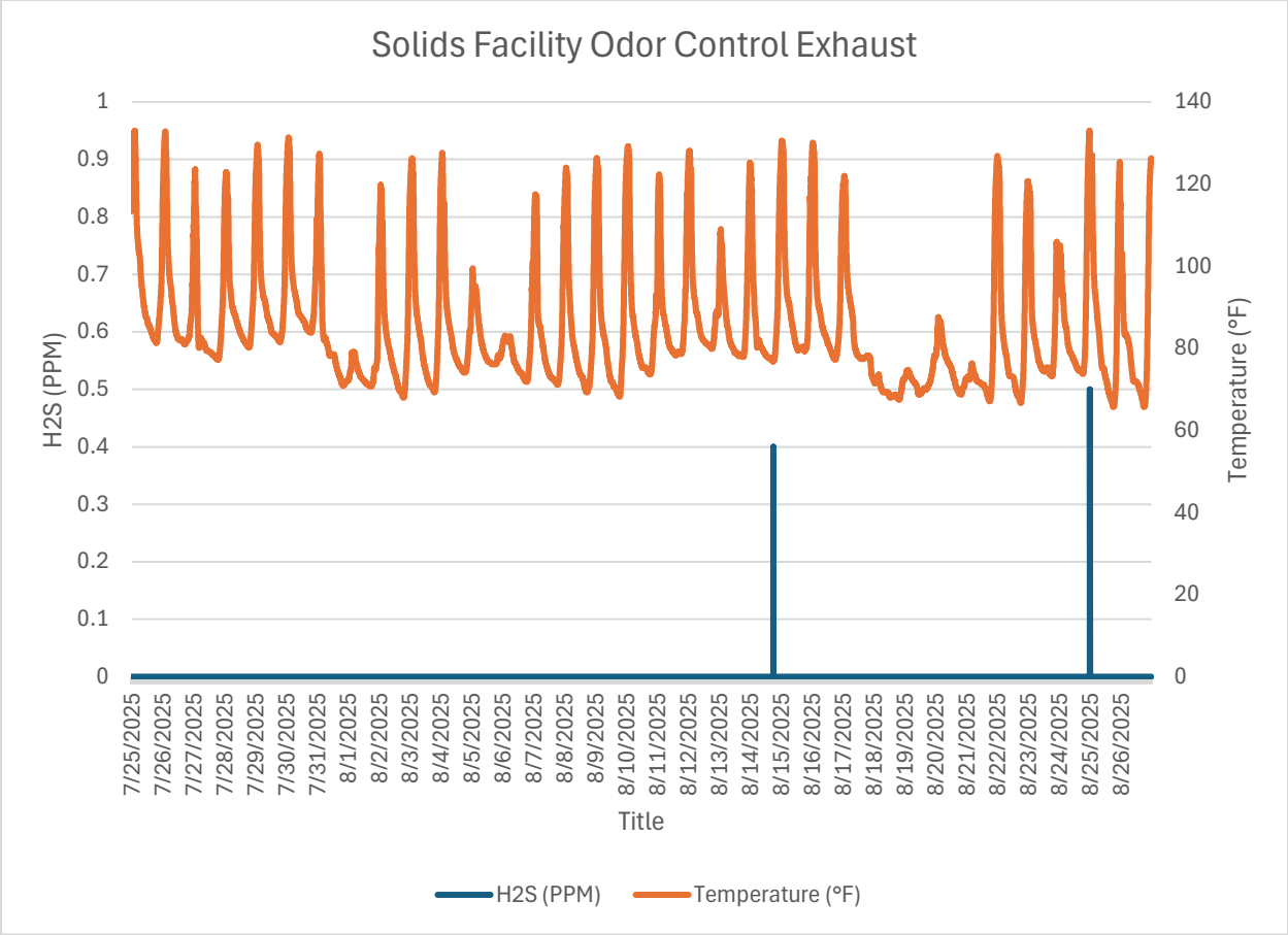
Monitor 6 Within WRF: Solids Facility Odor Control System Exhaust H2S PPM August, 2025
