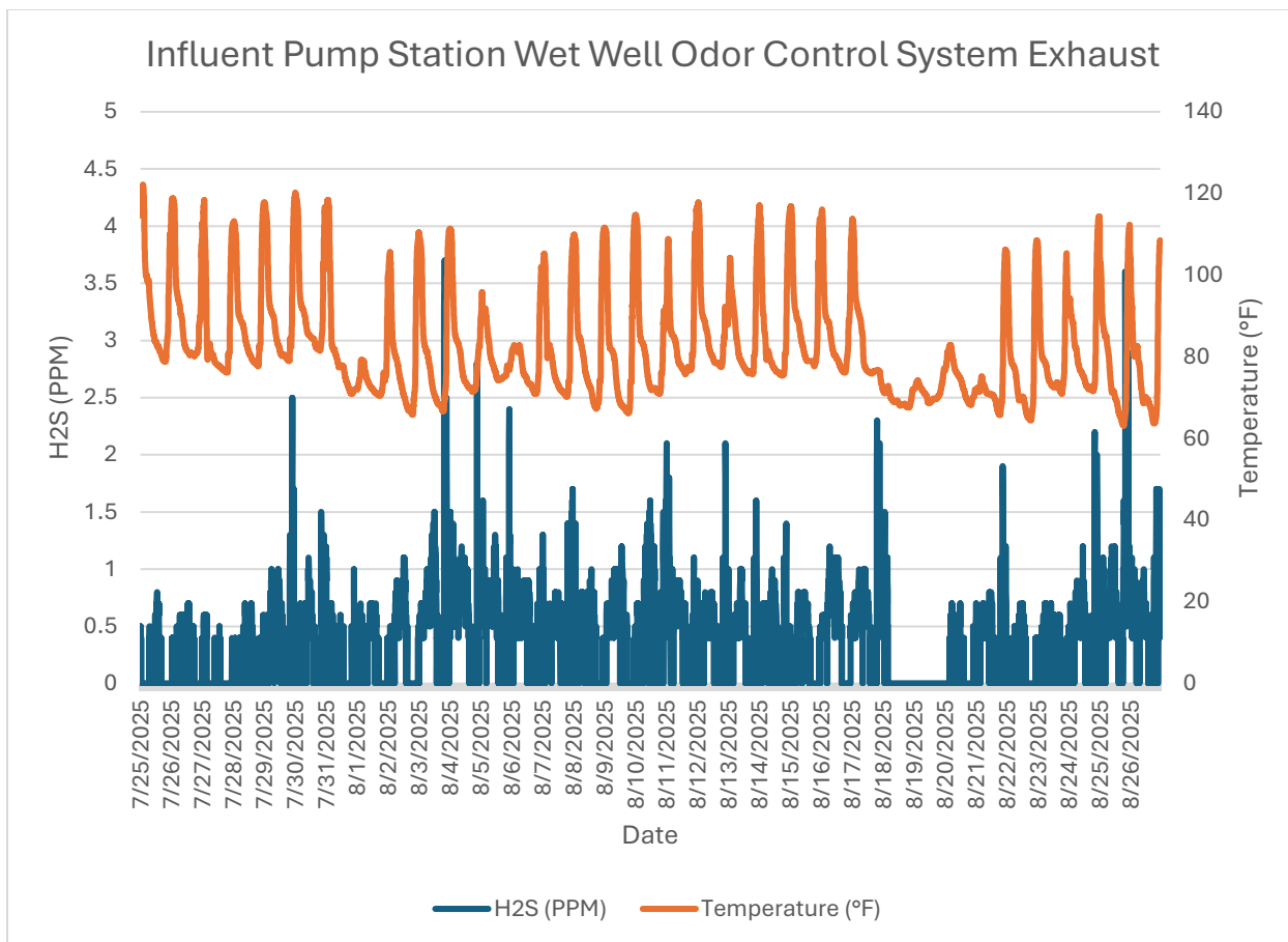
Monitor 1b Within WRF: Influent Pump Station Wet Well Odor Control System Exhaust H2S PPM August, 2025
