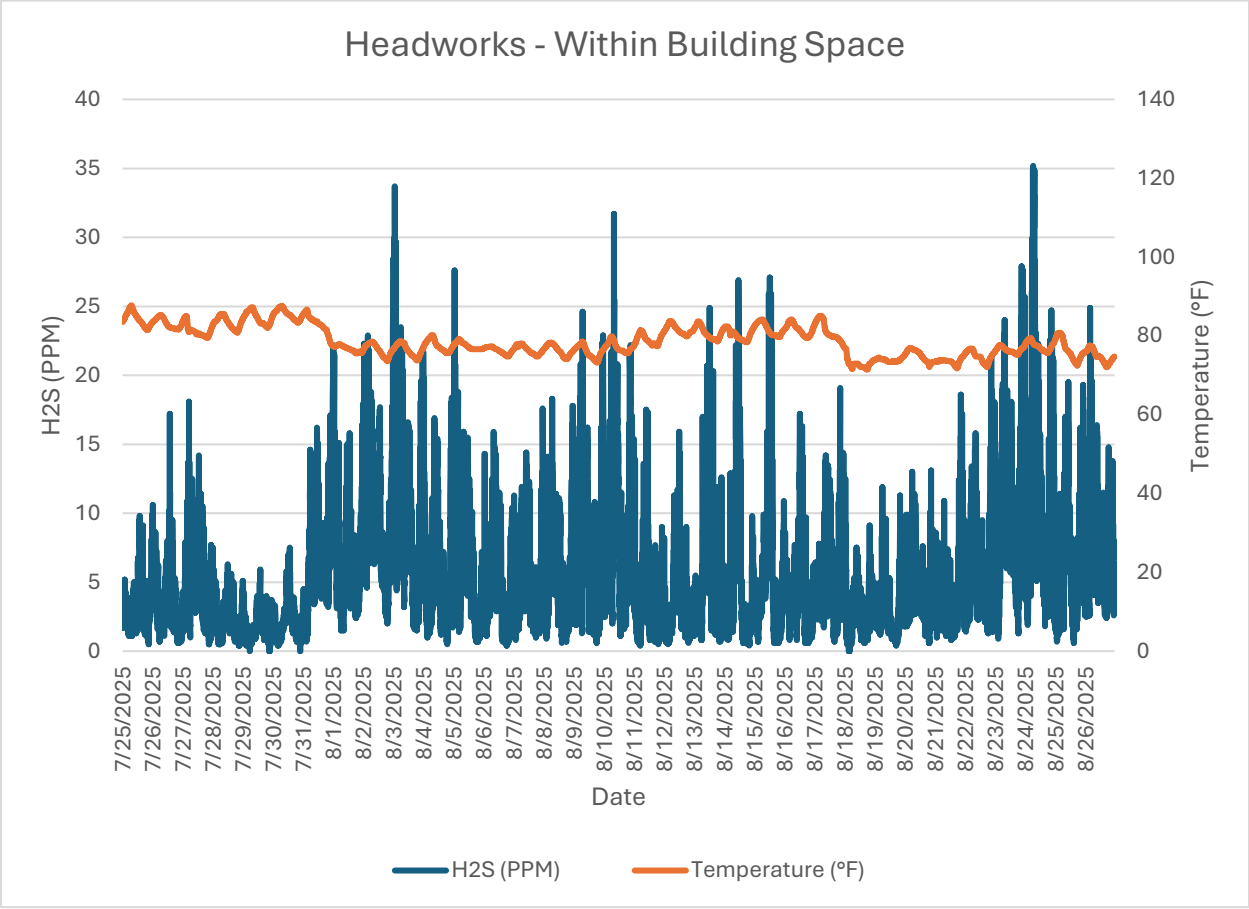
Monitor 2a Within WRF: Headworks – Within Building Space H2S PPM August, 2025
