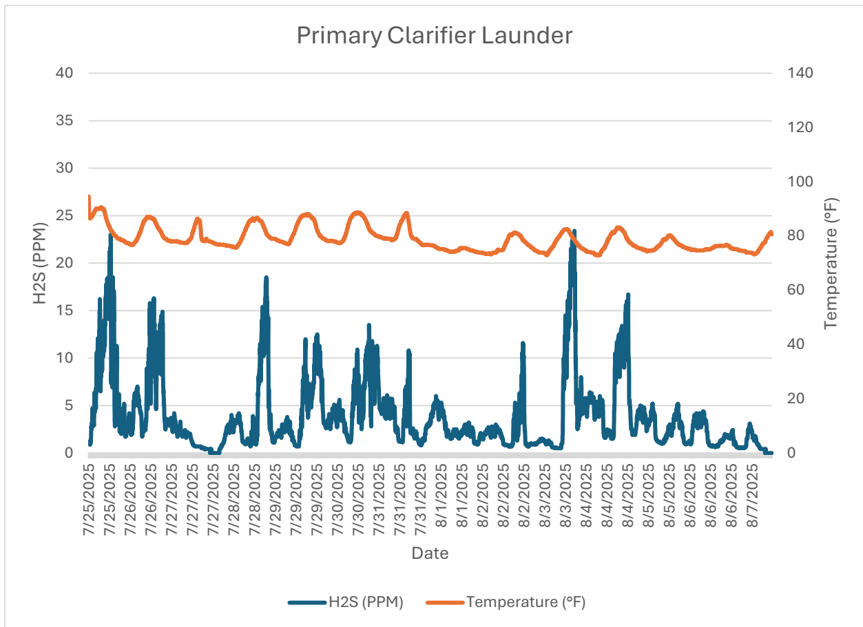
Monitor 3 Within WRF: Primary Clarifier Launder H2S PPM August, 2025 Monitor did not log from 8/7 to 8/14 see next page for rest of August data collected.
