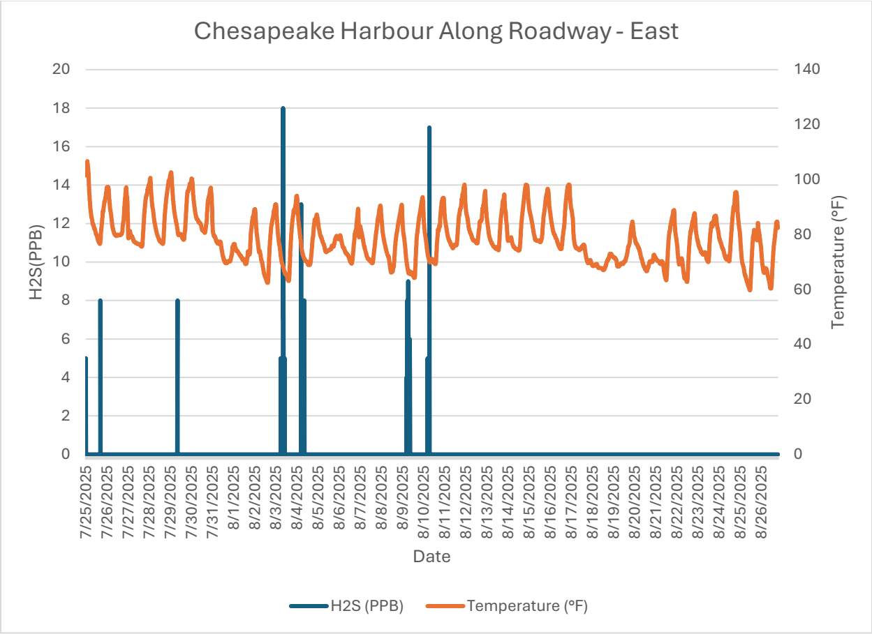
Monitor 5 Neighborhood Chesapeake Harbour Along Roadway - East H2S PPB August, 2025
