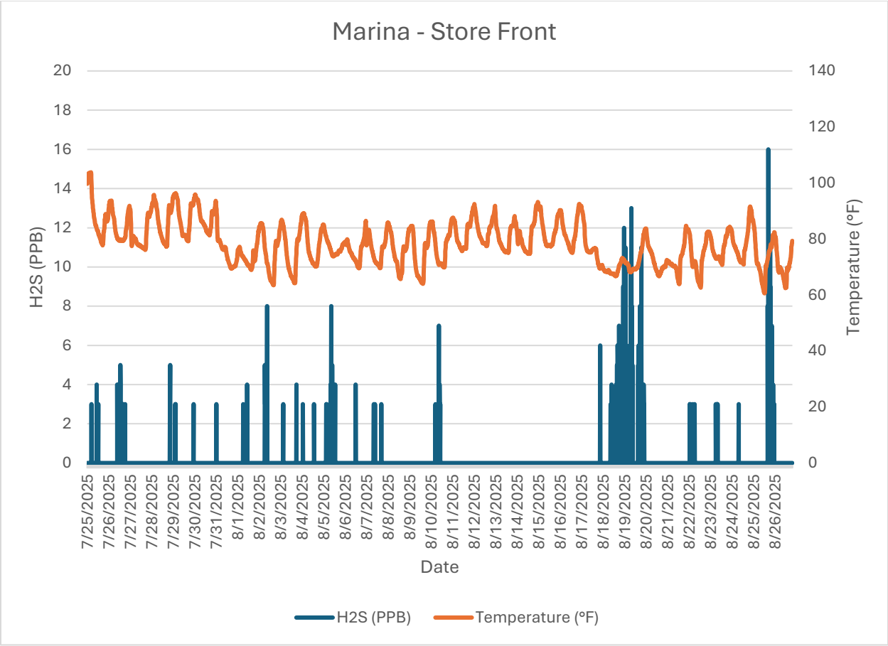
Monitor 1 Neighborhood: Marina – Store Front H2S PPB August, 2025
