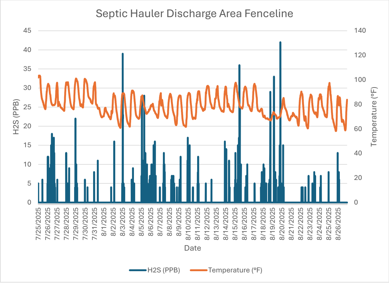
Monitor 1 Fenceline: Septic Discharge Area Fenceline H2S PPB August, 2025
