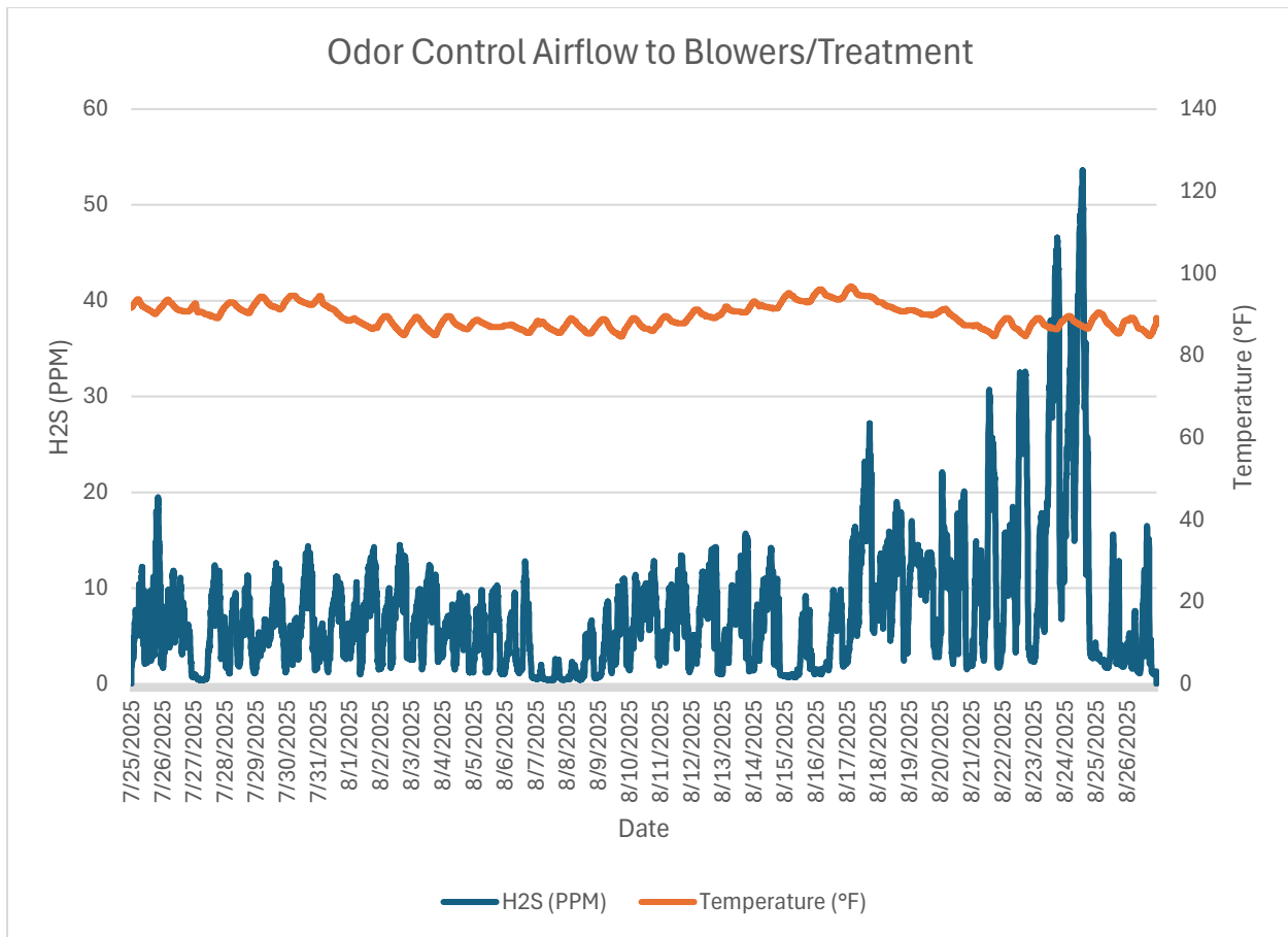
Monitor 4 Within WRF: Odor Control Airflow to Blowers/Treatment H2S PPM August, 2025
