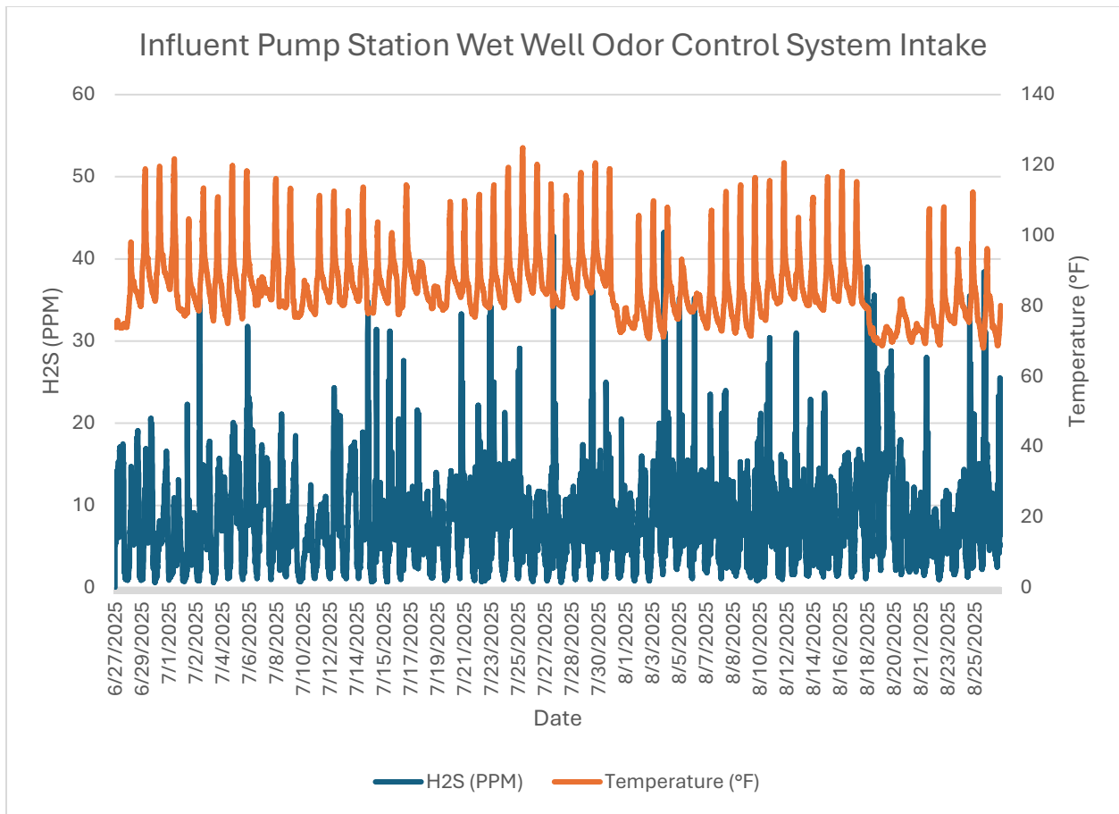
Monitor 1a Within WRF: Influent Pump Station Wet Well Odor Control System Intake H2S PPM July and August, 2025
