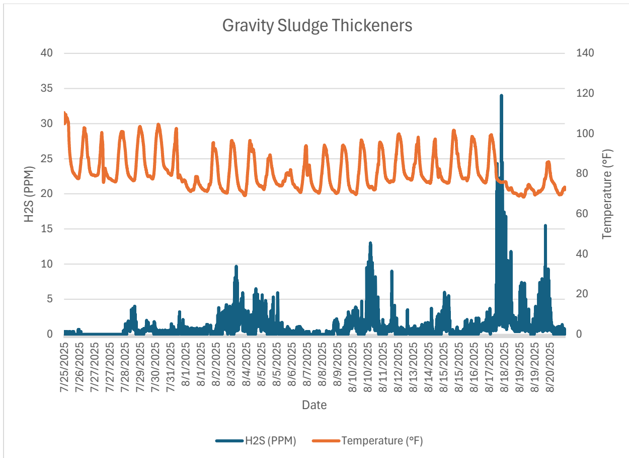
Monitor 5 Within WRF: Gravity Sludge Thickener H2S PPM August, 2025 Monitor got turned off on 8/21
