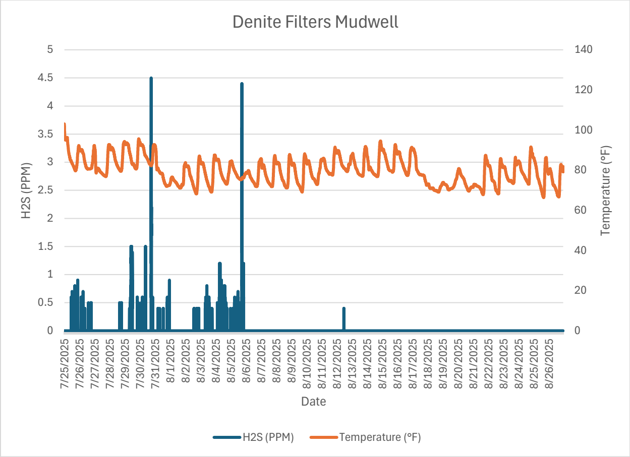
Monitor 7 Within WRF: Denite Filters Mudwell H2S PPM August, 2025
