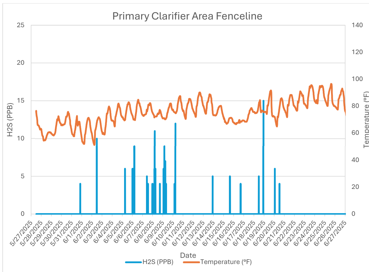
Monitor 2 Fenceline: Primary Clarifier Area Fenceline H2S PPB June, 2025
