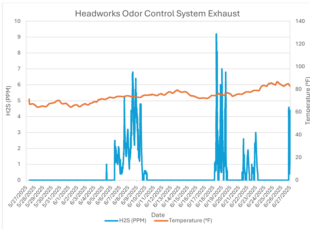
Monitor 2b Within WRF: Headworks Odor Control System Exhaust H2S PPM June, 2025
