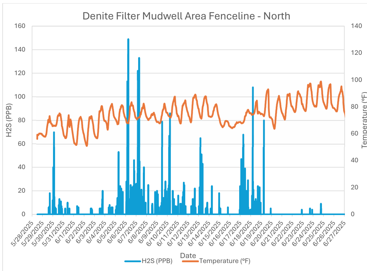
Monitor 3 Fenceline: Denite Filter Mudwell Area Fenceline- North H2S PPB June, 2025
