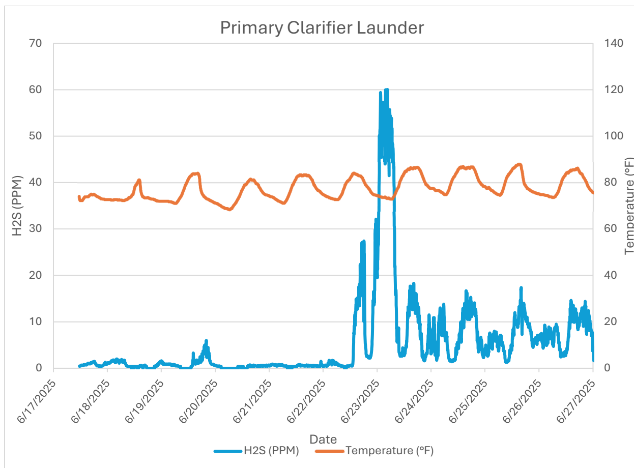
Monitor 3 Within WRF: Primary Clarifier Launder H2S PPM June, 2025
