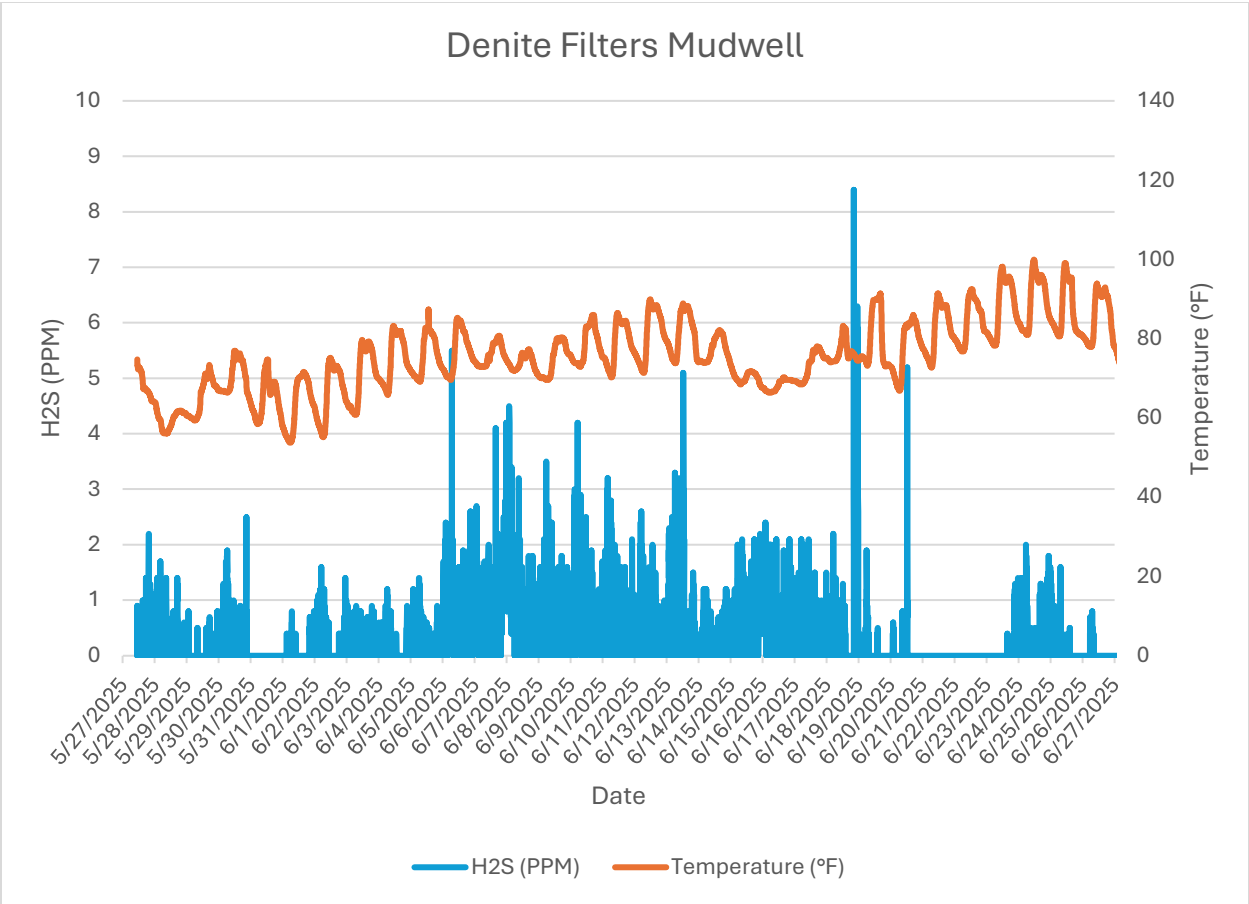
Monitor 7 Within WRF: Denite Filters Mudwell H2S PPM June, 2025
