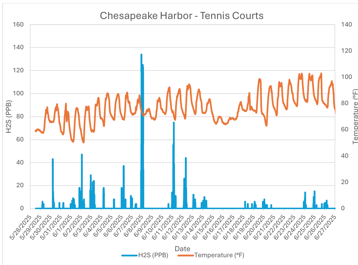
Monitor 4 Neighborhood Chesapeake Harbor – Tennis Courts H2S PPB June, 2025
