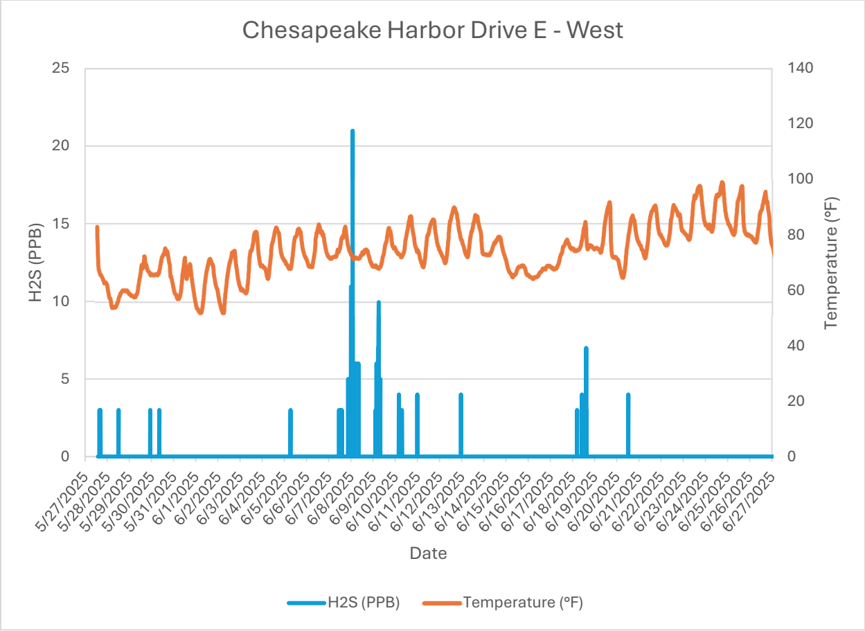
Monitor 6 Neighborhood Chesapeake Harbor Drive E - West H2S PPB June, 2025
