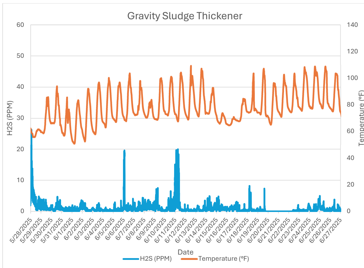
Monitor 5 Within WRF: Gravity Sludge Thickener H2S PPM June, 2025
