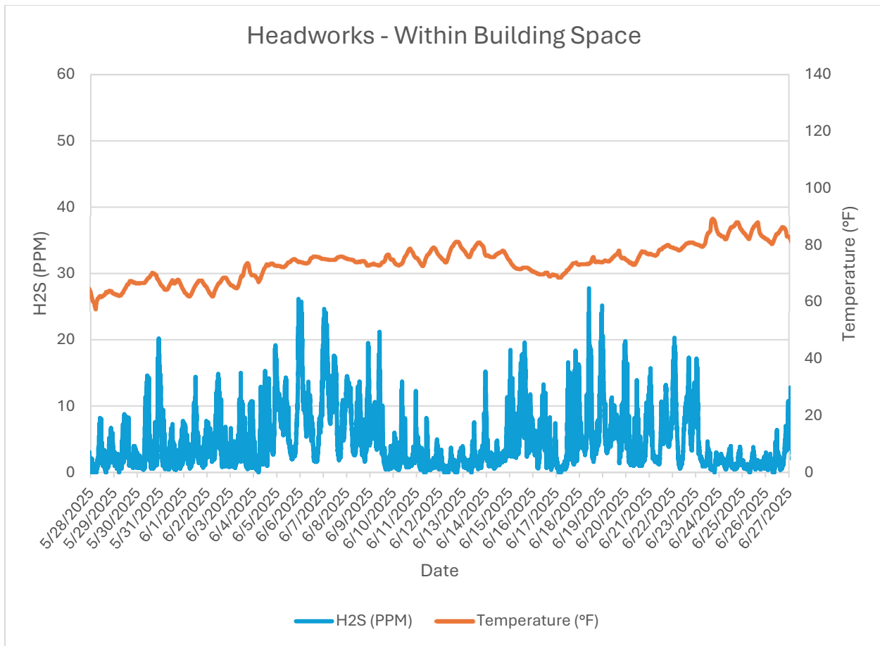
Monitor 2a Within WRF: Headworks – Within Building Space H2S PPM June, 2025
