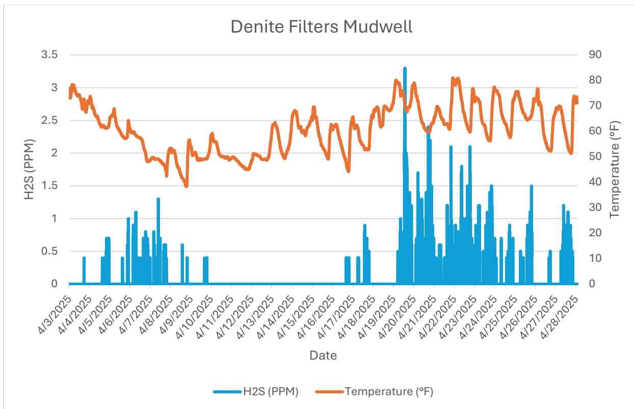
Monitor 7 Within WRF: Denite Filters Mudwell H2S PPM April, 2025
