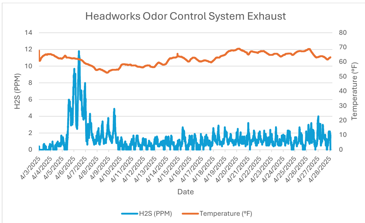
Monitor 2b Within WRF: Headworks Odor Control System Exhaust H2S PPM April, 2025
