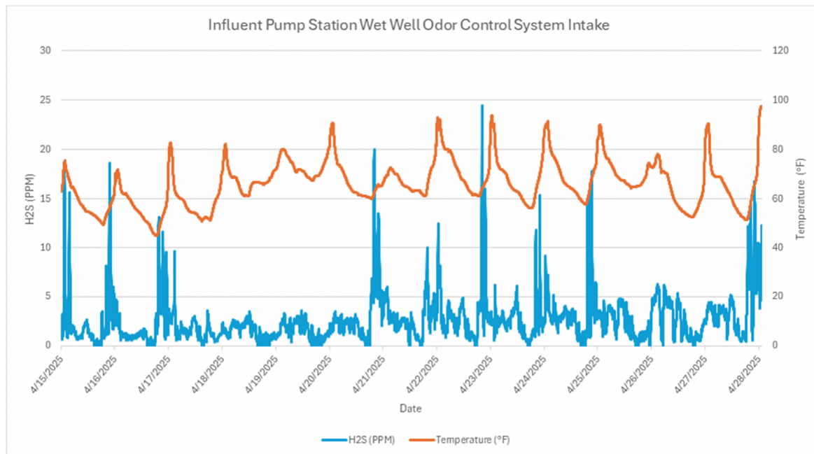
Monitor 1a Within WRF: Influent Pump Station Wet Well Odor Control System Intake H2S PPM April, 2025
