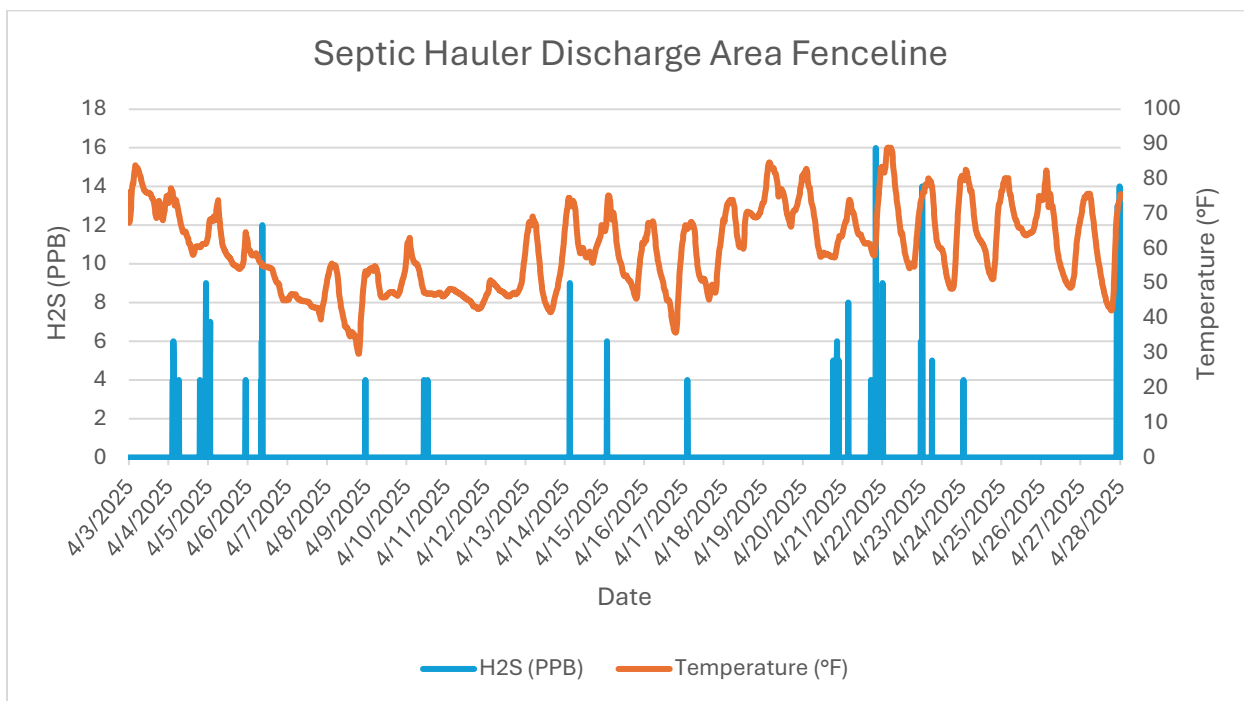
Monitor 1 Fenceline: Septic Hauler Discharge Area Fenceline H2S PPB April, 2025
