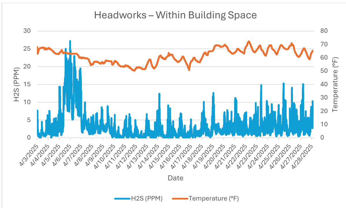
Monitor 2a Within WRF: Headworks – Within Building Space H2S PPM April, 2025
