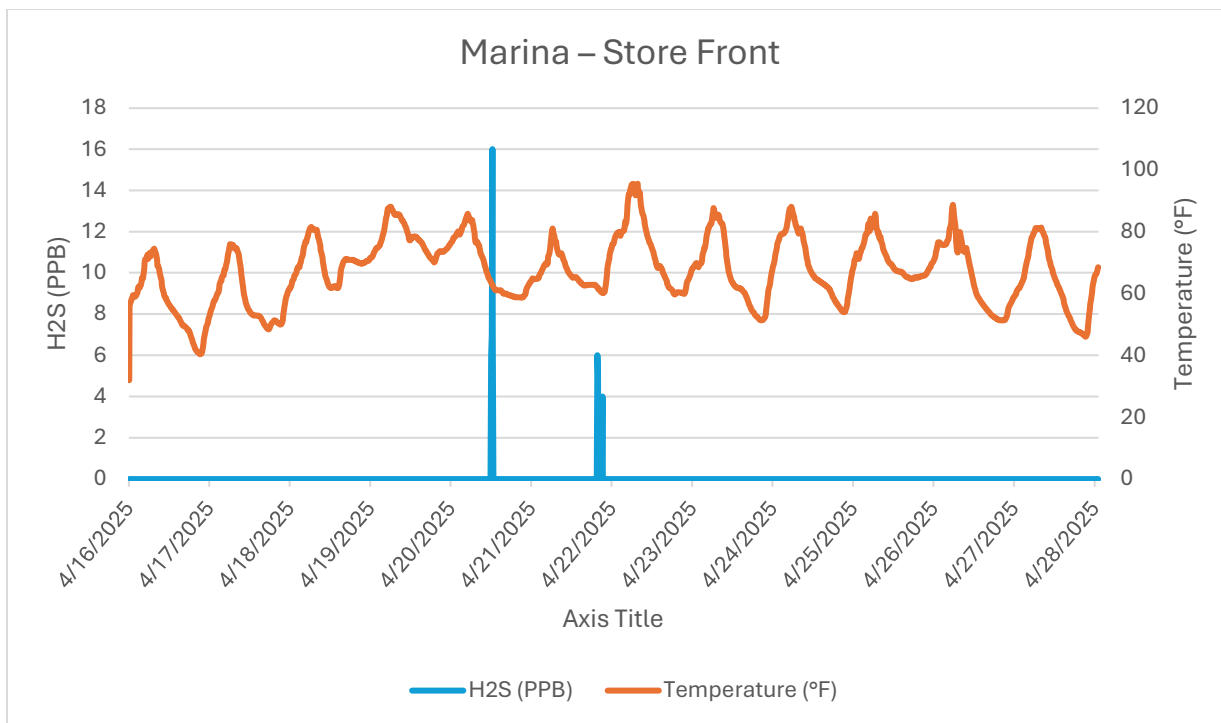
Monitor 1 Neighborhood: Marina – Store Front H2S PPB April, 2025 (Note- estimated dates adjusted per display issue)
