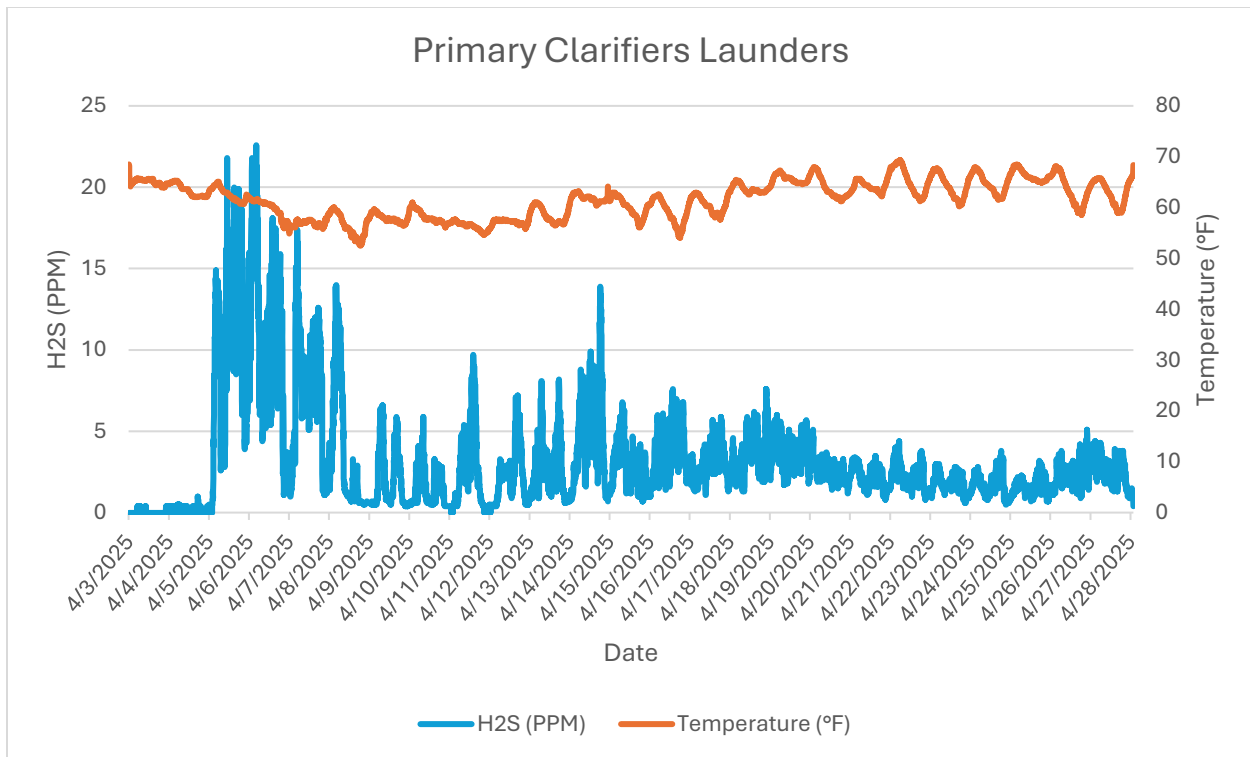
Monitor 3 Within WRF: Primary Clarifier Launder H2S PPM April, 2025
