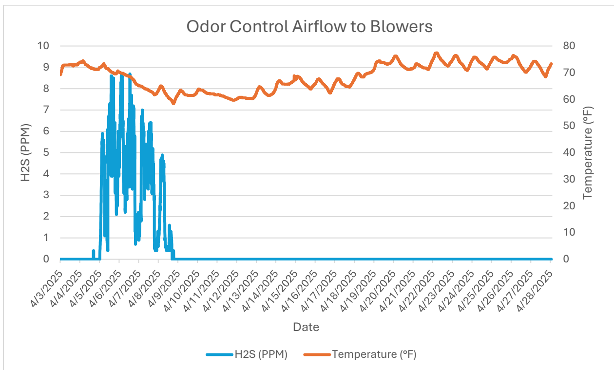
Monitor 4 Within WRF: Odor Control Airflow to Blowers/Treatment H2S PPM April, 2025
