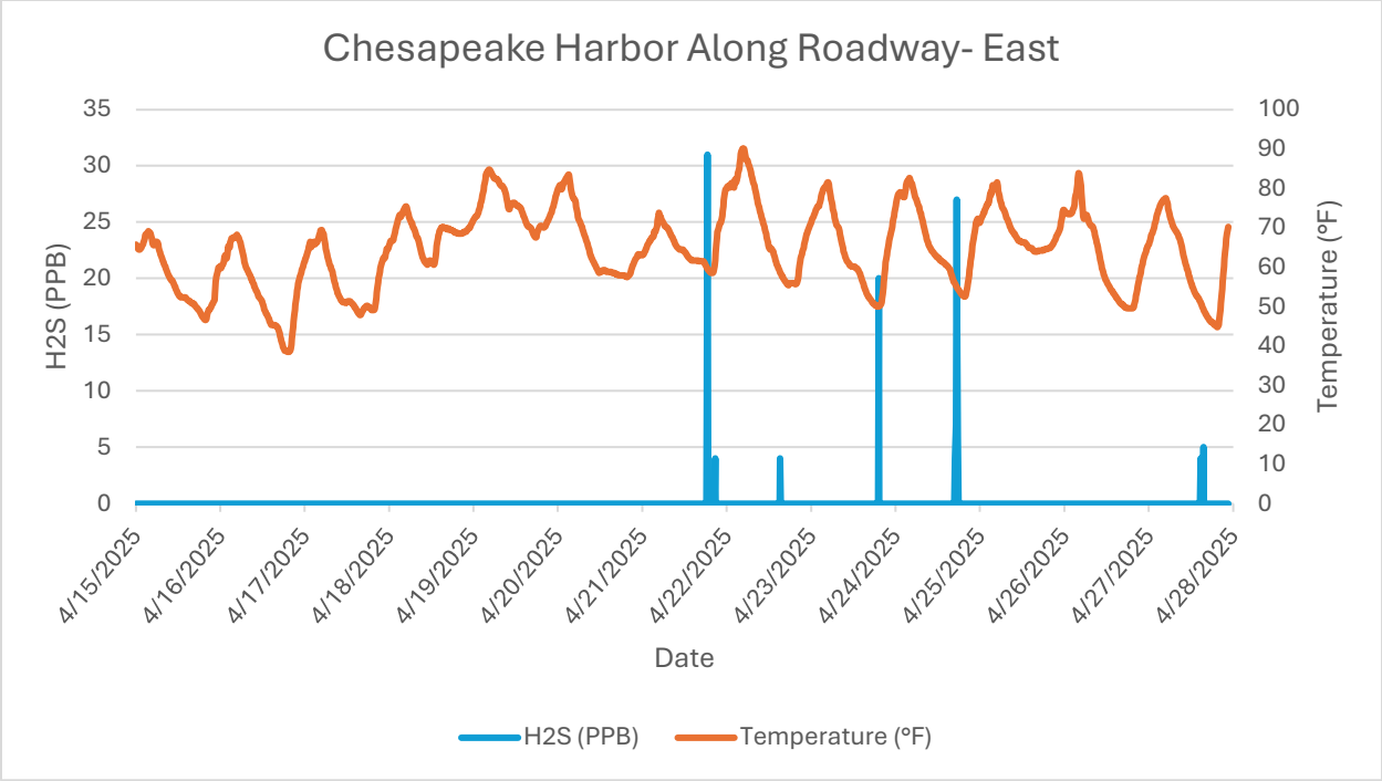
Monitor 5 Neighborhood: Chesapeake Harbor along roadway H2S PPB
