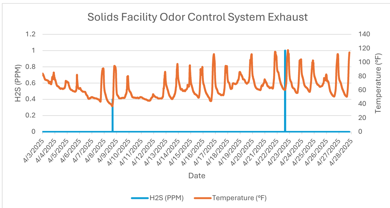
Monitor 6 Within WRF: Solids Facility Odor Control System Exhaust H2S PPM April, 2025
