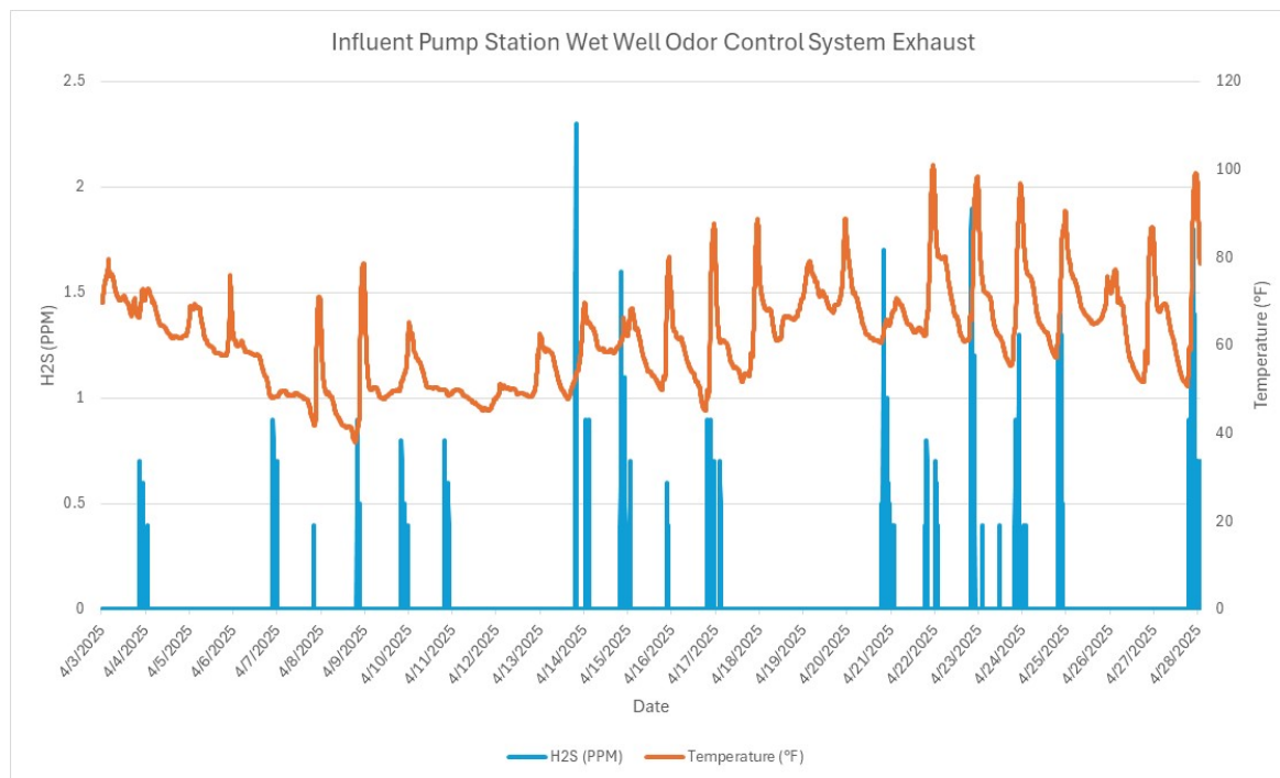
Monitor 1b Within WRF: Influent Pump Station Wet Well Odor Control System Exhaust H2S PPM April, 2025
