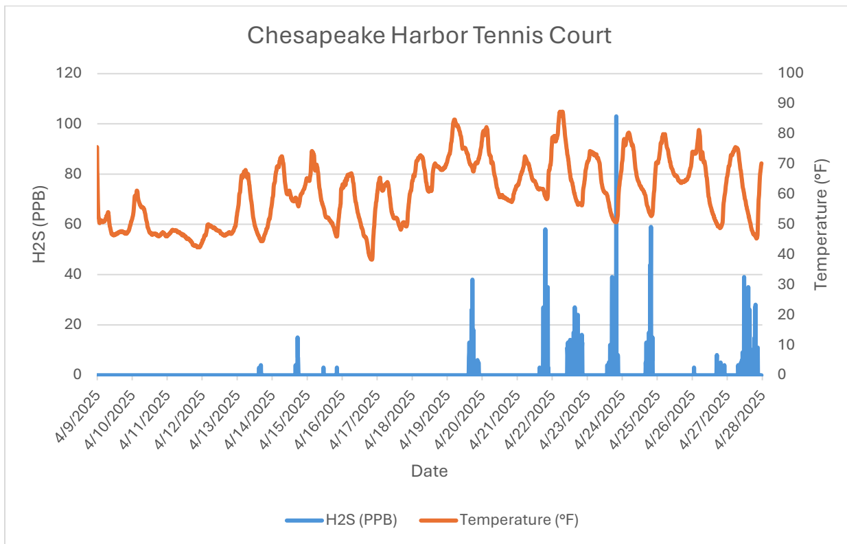
Monitor 4 Neighborhood: Chesapeake Harbor Tennis Court H2S PPB April, 2025
