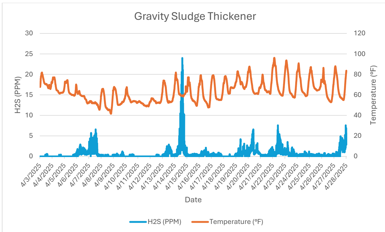
Monitor 5 Within WRF: Gravity Sludge Thickener H2S PPM April, 2025
