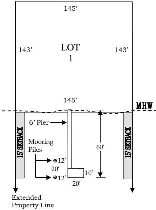
90° Angle to the Shoreline
