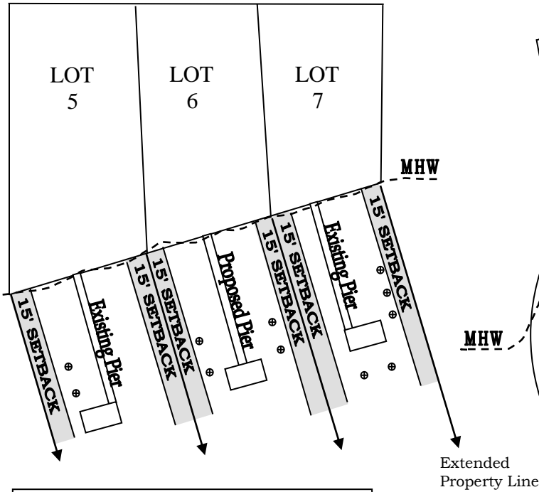
Generally Parallel with Existing Piers on Adjacent Lots
