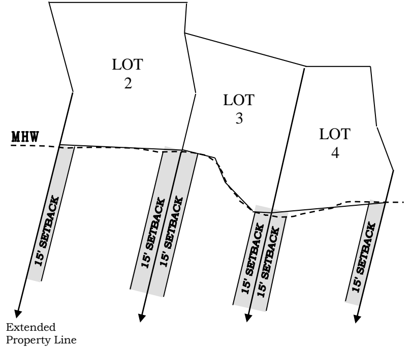
Extension of the Last Course of the Lot Line
