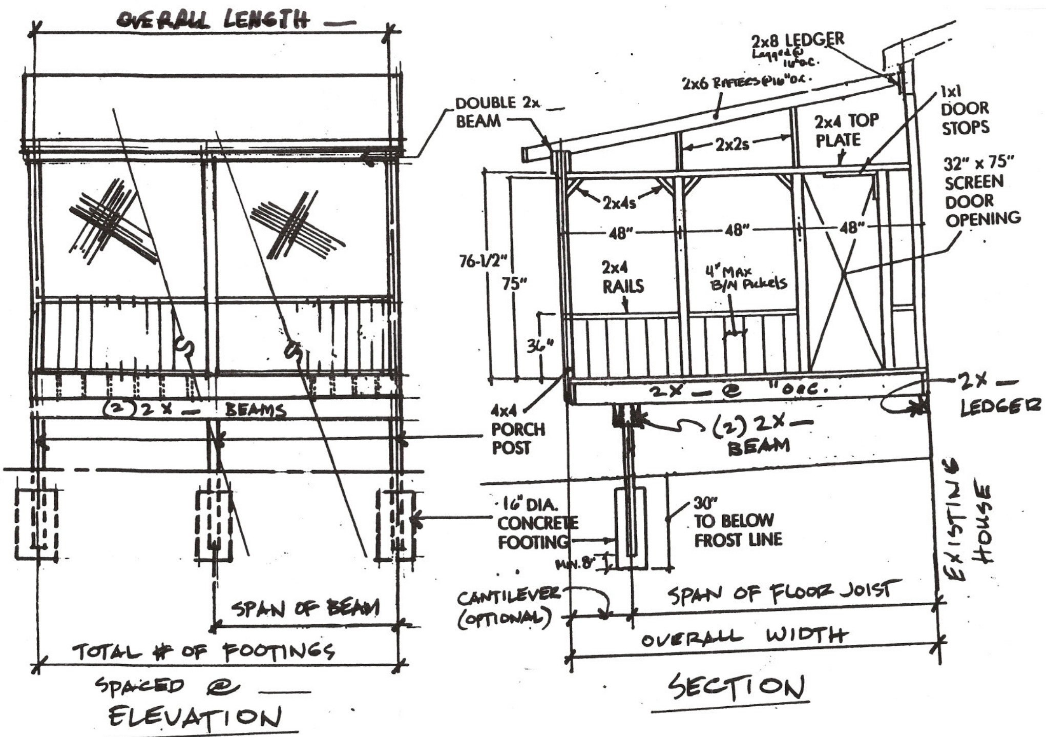
Typical Screen Porch
