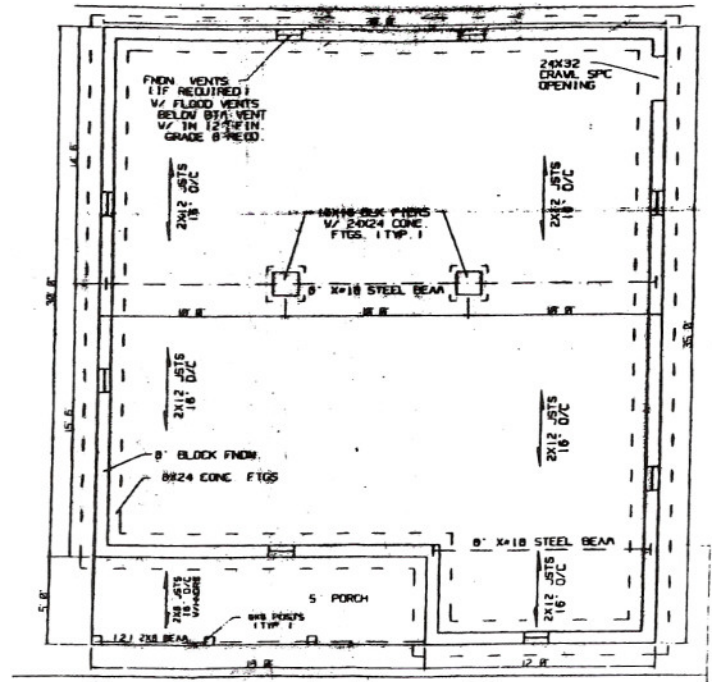
B Foundation Plan
