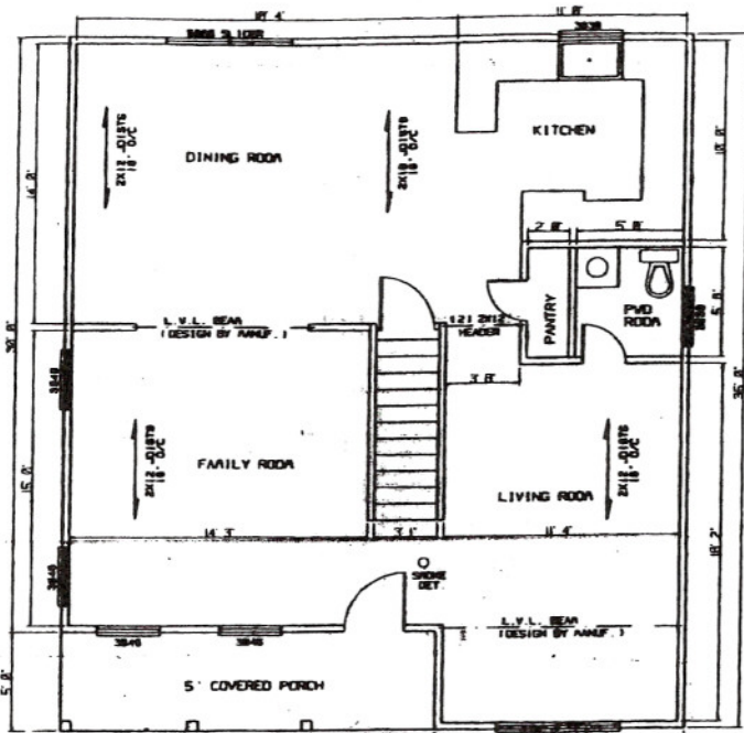
A Floor Plan
